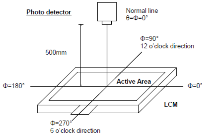
Optical measurement system setup
