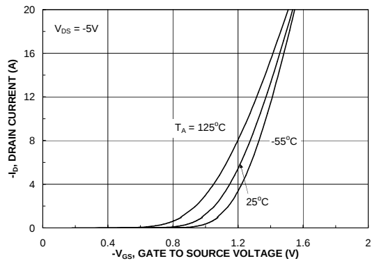
Figure 16. Transfer Characteristics.
