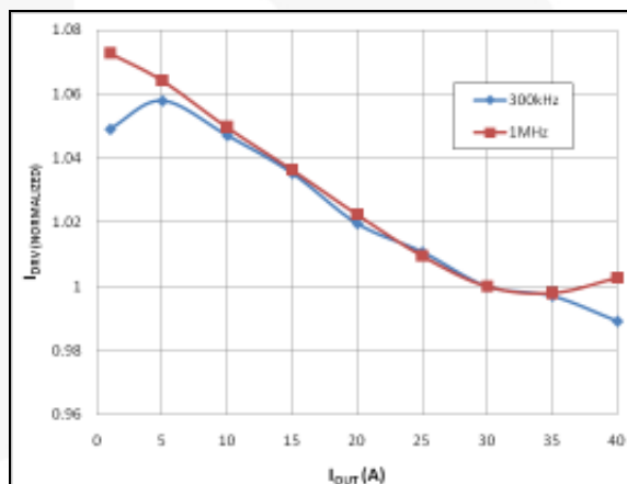
Figure 15. Driver Supply Current vs. Output Current
