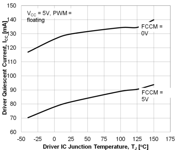
Figure 24. Driver Quiescent Current vs. Temperature
