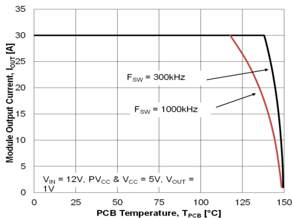
Figure 4. Safe Operating Area with 12 V_{IN}
