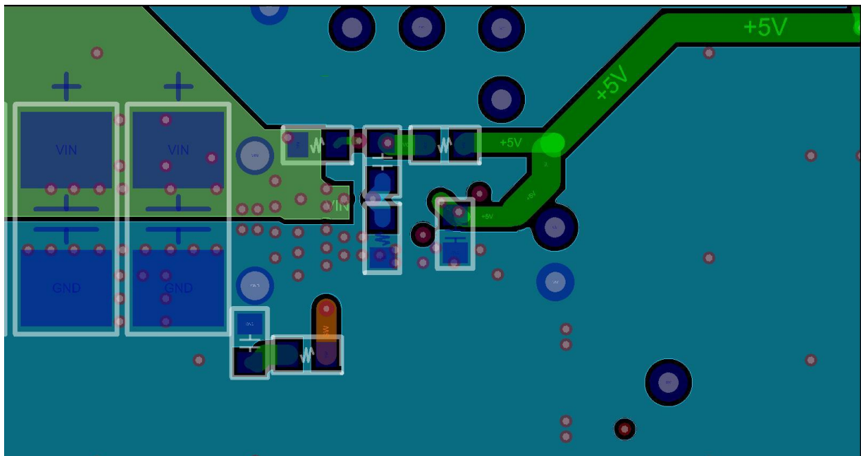
Figure 33. Single-Phase Board Layout Example – Bottom View (Mirrored)
