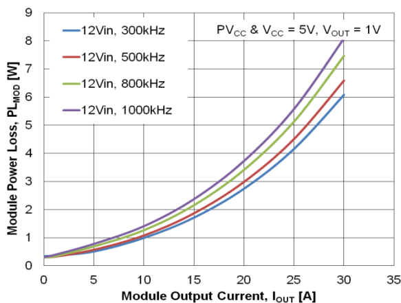
Figure 6. Power Loss vs. Output Current with 12 V_{IN}
