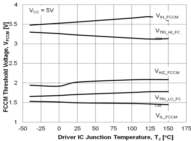
Figure 20. FCCM Threshold vs. Temperature
