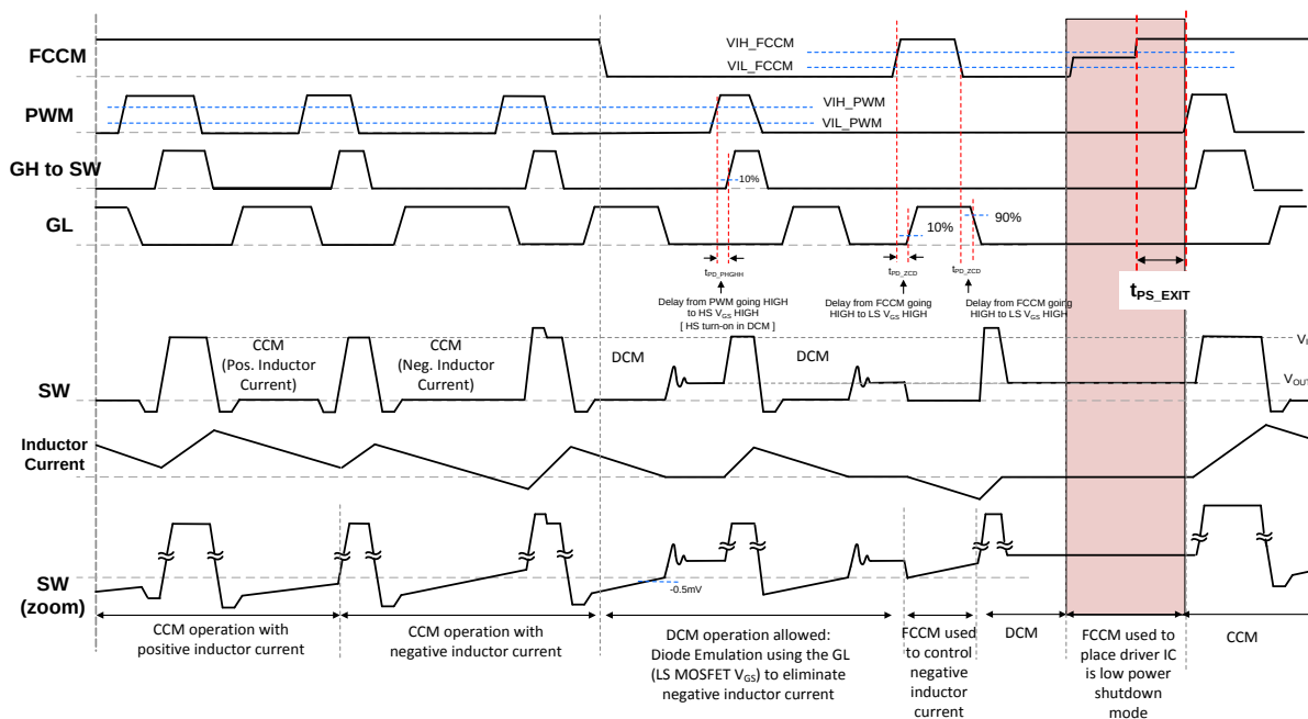
Figure 30. FCCM 3-State Timing Diagram
