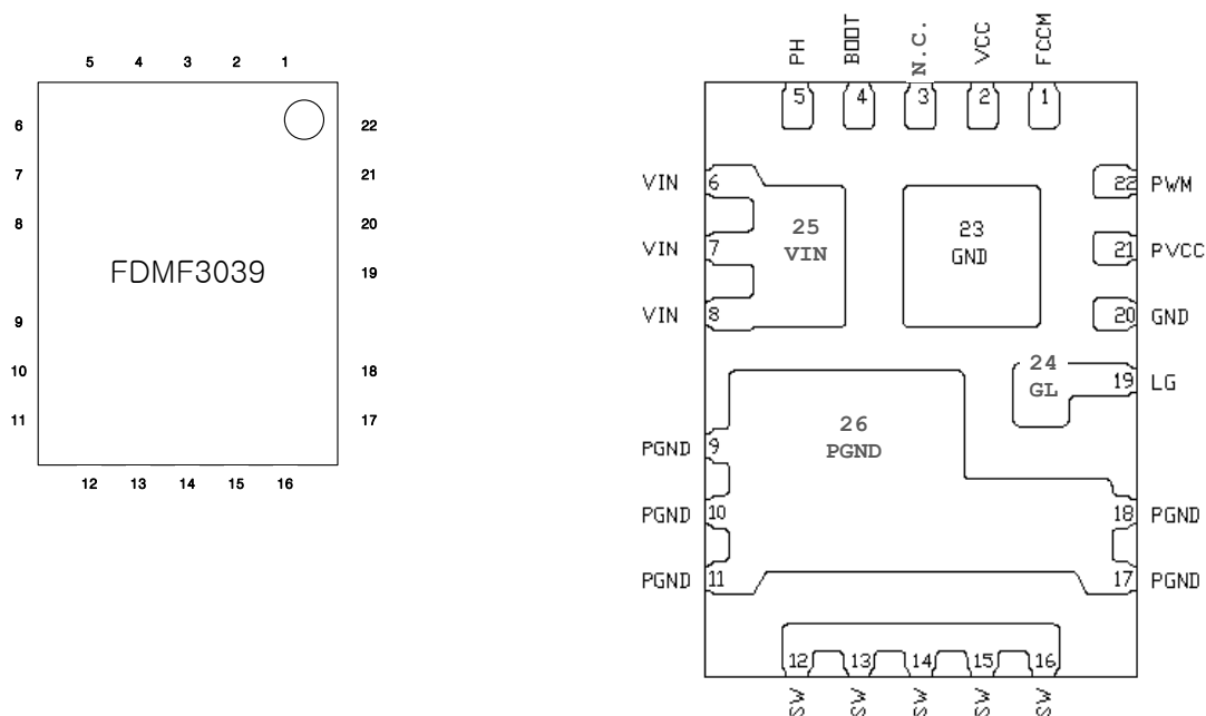
Figure 3. Pin Configuration - Top View and Transparent View
