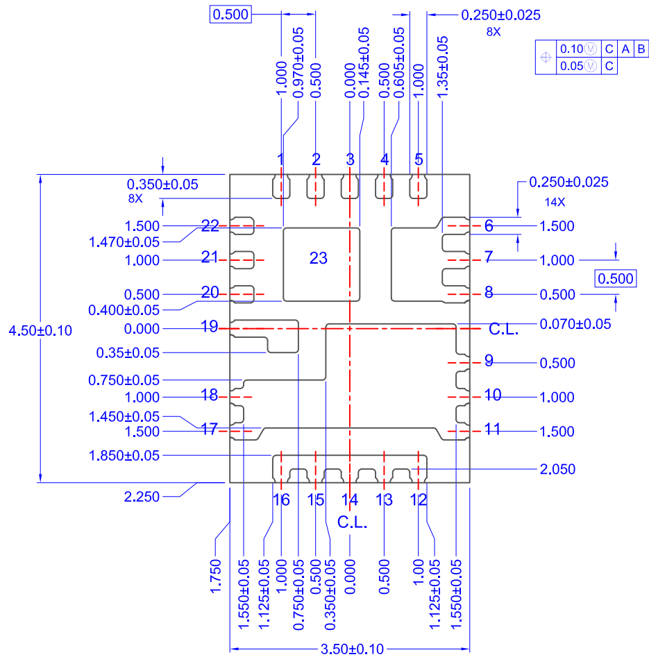
BOTTOM VIEW
