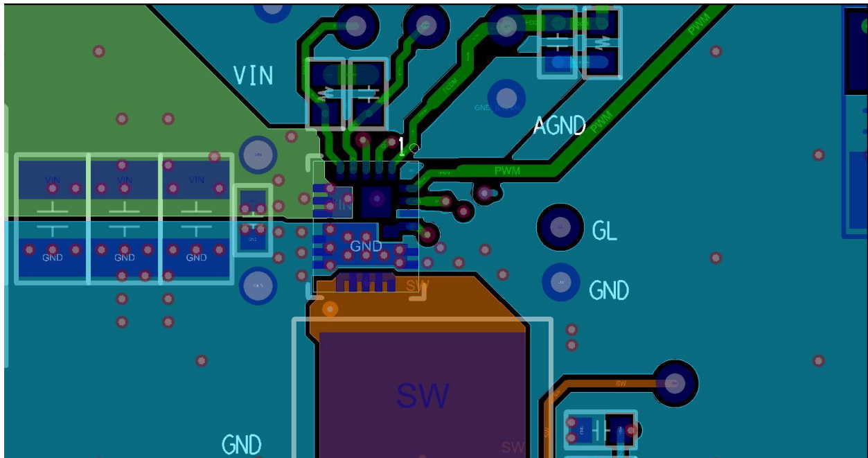
Figure 32. Single-Phase Board Layout Example – Top View
