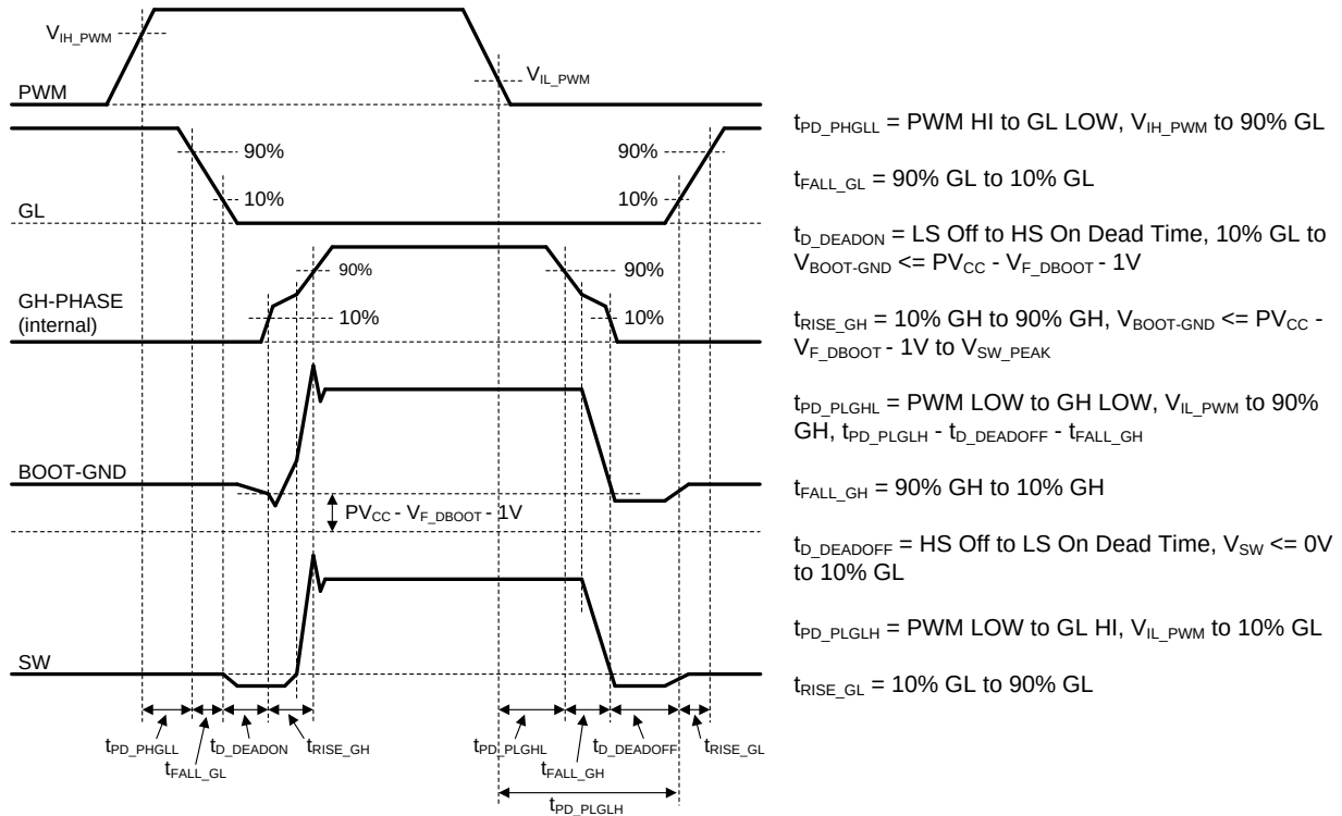
Figure 26. PWM Timing Diagram
