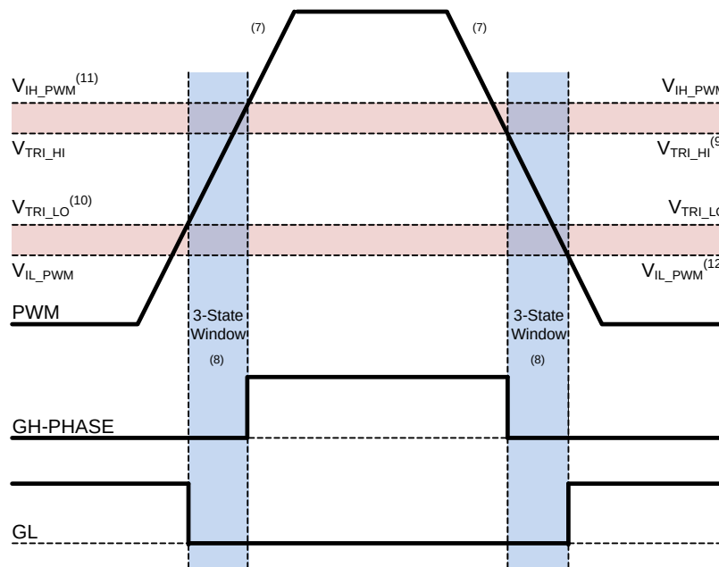
Figure 27. PWM Threshold Definition
