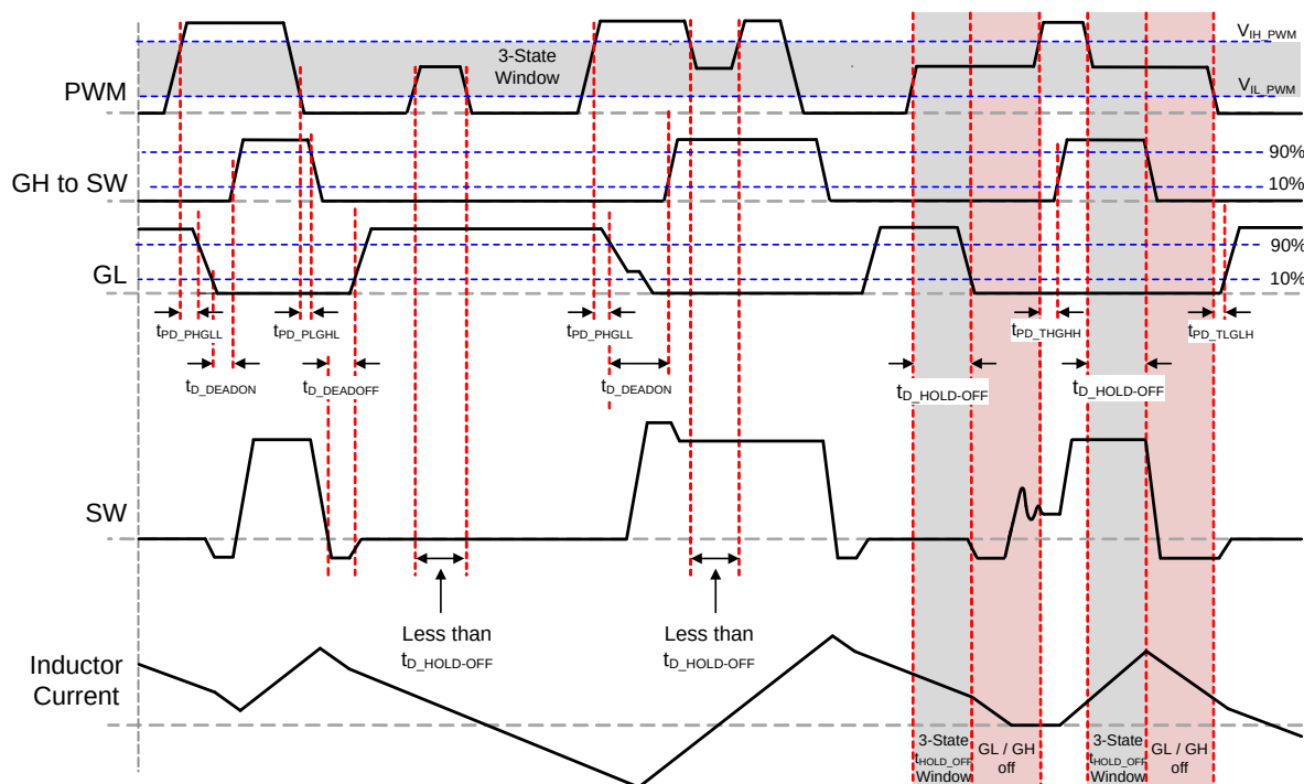
Figure 29. PWM 3-State Timing Diagram (FCCM held HIGH)
