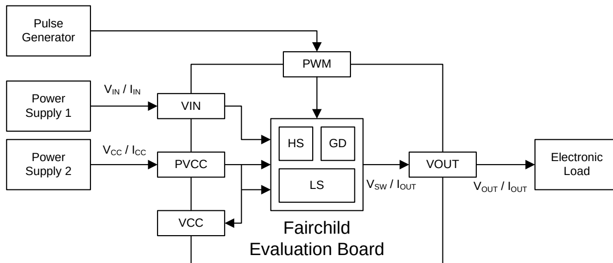
Figure 31. Power Loss and Efficiency Measurement Diagram
