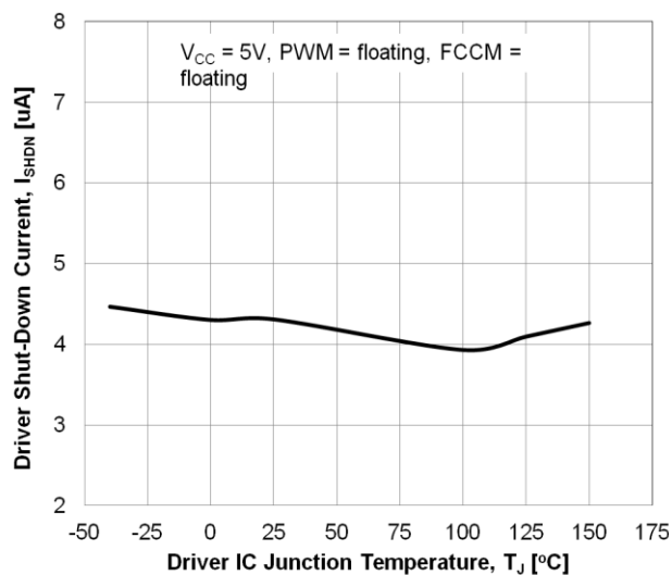
Figure 23. Driver Shutdown Current vs. Temperature
