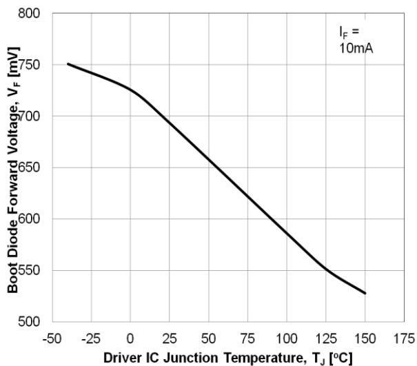
Figure 22. Boot Diode Forward Voltage vs. Temperature
