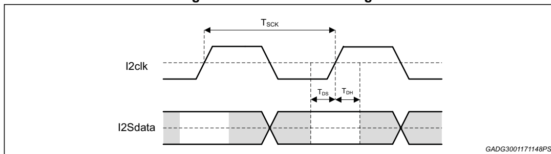
Figure 67. I 2 S Interface timings
