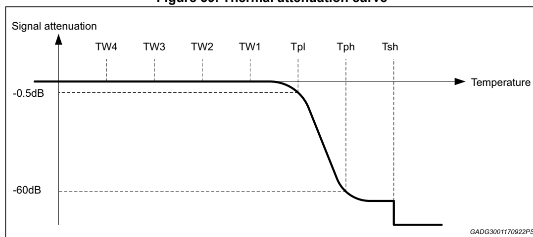
Figure 59. Thermal attenuation curve
