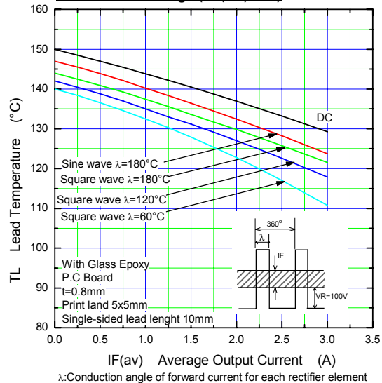
Current Derating ( I_F(\text{av}) -TL)
