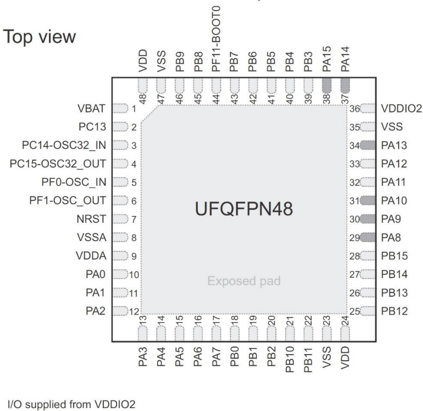
FCM32x042 UFQFPN48 pinout
