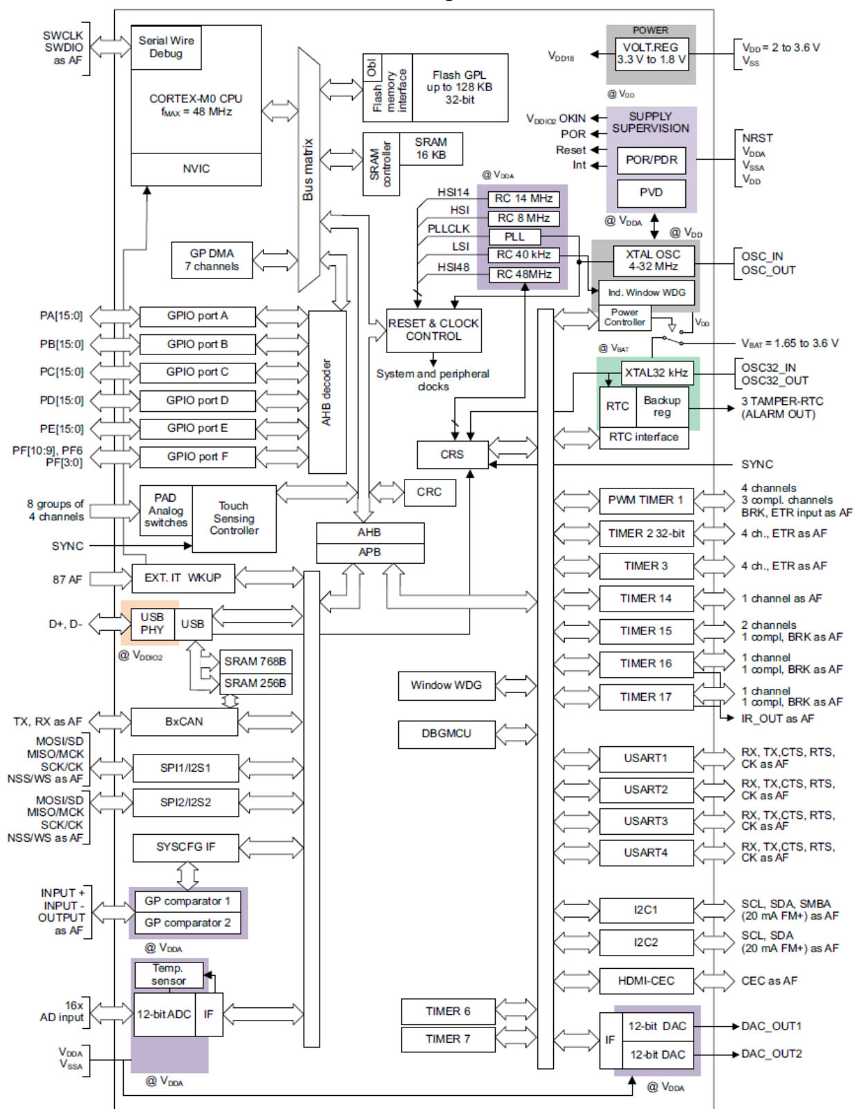
Block diagram
