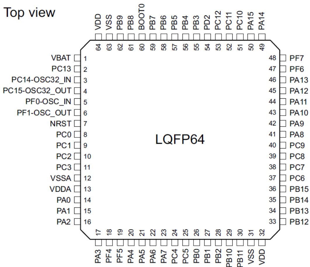
FCM32F051 LQFP64 pinout
