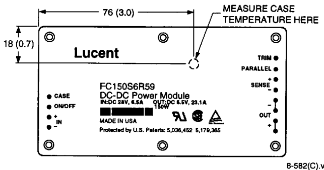
Figure 16. Case Temperature Measurement Location
