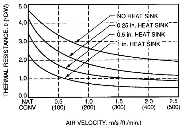
Figure 19. Heat Sink Resistance Curves; Fins Oriented Along Length
