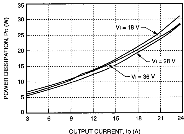
Figure 20. Power Dissipation as Heat vs. Output Current
