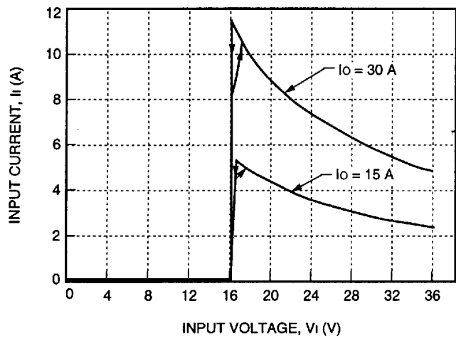
Figure 1. Typical FC150S6R5 Input Characteristics at Room Temperature
