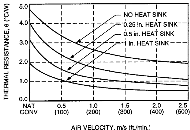
Figure 18. Heat Sink Resistance Curves; Fins Oriented Along Width
