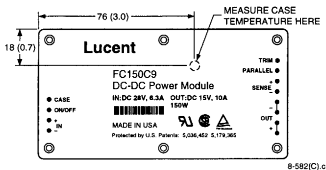
Figure 17. Case Temperature Measurement Location
