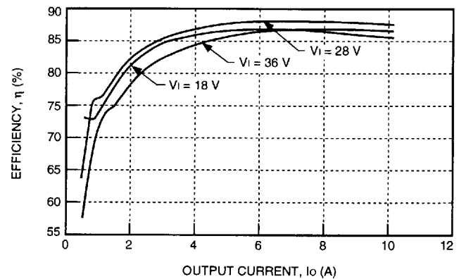
Figure 3. Typical FC150C Efficiency vs. Output Current at Room Temperature
