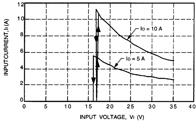
Figure 1. Typical FC150C Input Characteristics at Room Temperature
