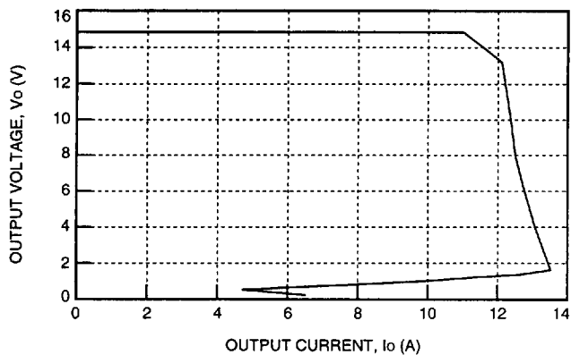
Figure 2. Typical FC150C Output Characteristics at Room Temperature and 28 V Input
