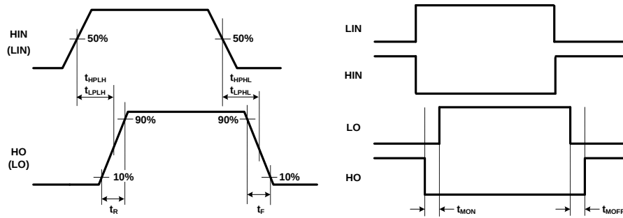
Figure 23. Timing Diagrams
