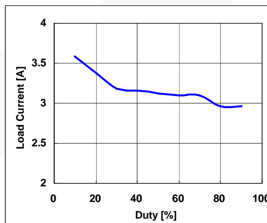
Figure 15. Current Limited Level vs. Duty Ratio
