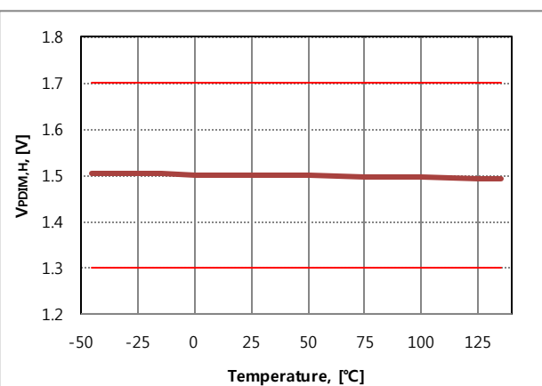
Figure 16. PWM Dimming Input High Voltage vs. Temperature
