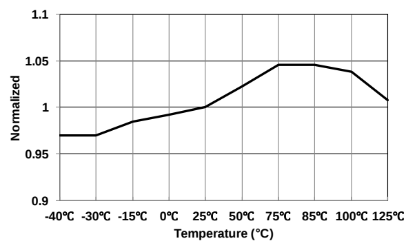
Figure 18 During of V_{SD-TH-ST} at startup ( t_{SD-ST} ) vs. Temperature
