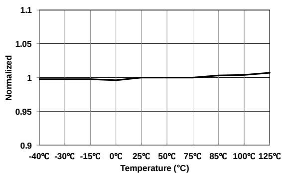
Figure 4 Turn-Off Threshold Voltage ( V_{DD-OFF} ) vs. Temperature
