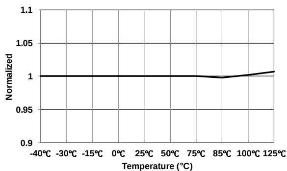
Figure 6 Brown-In Threshold Voltage ( V_{Brown-IN} ) vs. Temperature
