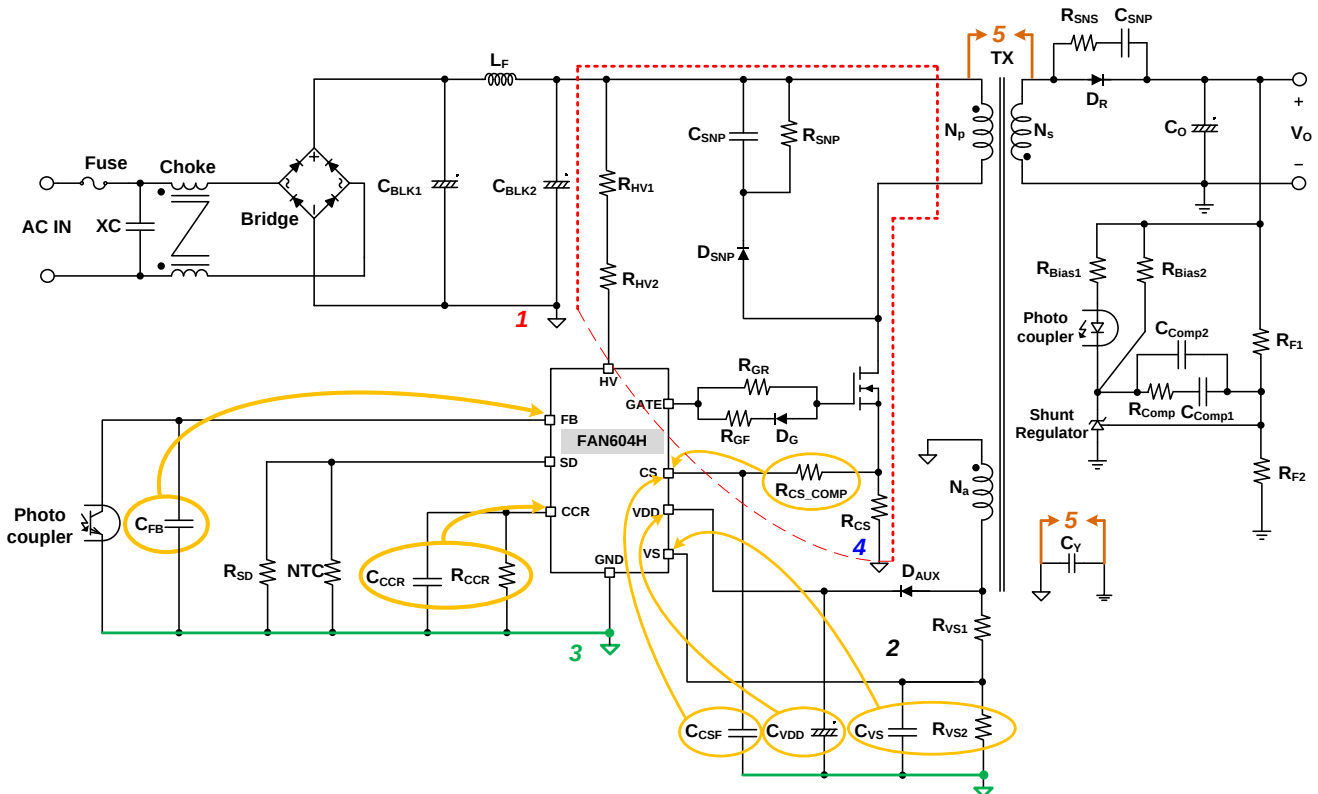
Figure 39 Recommended Layout for FAN604H
