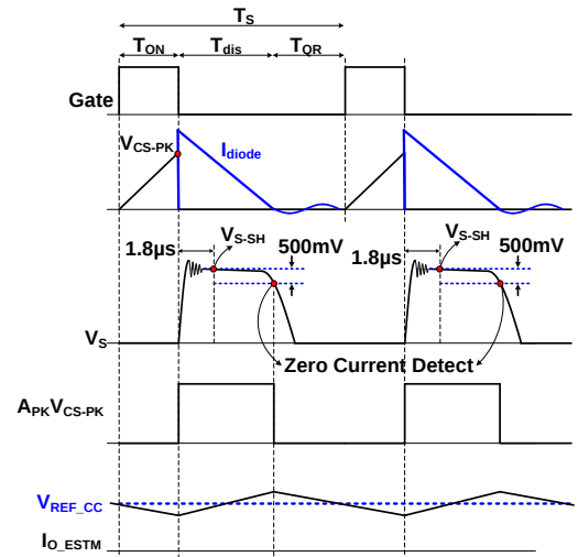
Figure 28 Waveforms for Estimate Output Current
