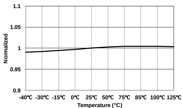
Figure 8 Minimum Blanking Frequency ( f_{BNK-MIN} ) vs. Temperature
