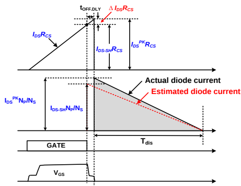
Figure 29 Effect of MOSFET Turn-off Delay and Line Voltage Compensation
