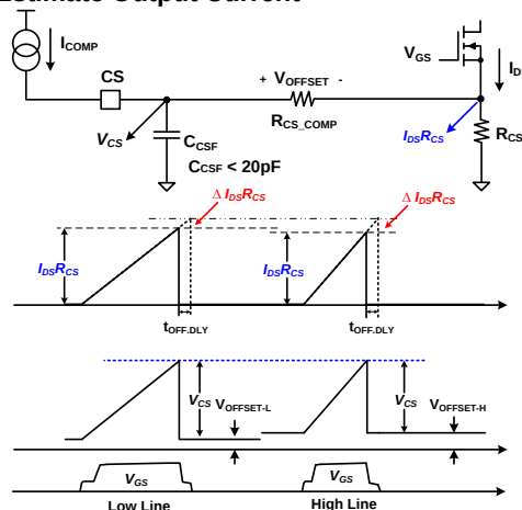
Figure 29 Effect of MOSFET Turn-off Delay and Line Voltage Compensation
