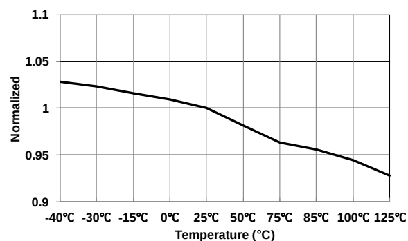
Figure 16 High Threshold Voltage of Current Sense ( V_{CS-IMIN-H} ) vs. Temperature
