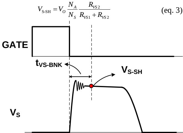
Figure 26 Output Voltage Detection
