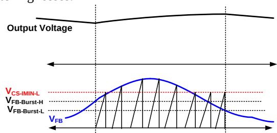
Figure 21 Burst-Mode Operation
