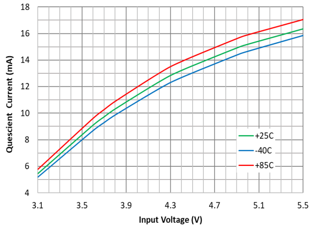
Figure 11. PWM Quiescent Current vs. Input Voltage and Temperature
