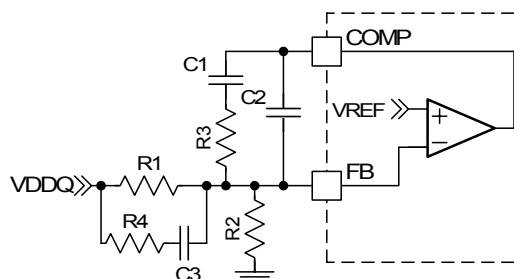
Figure 12. Compensation Network
