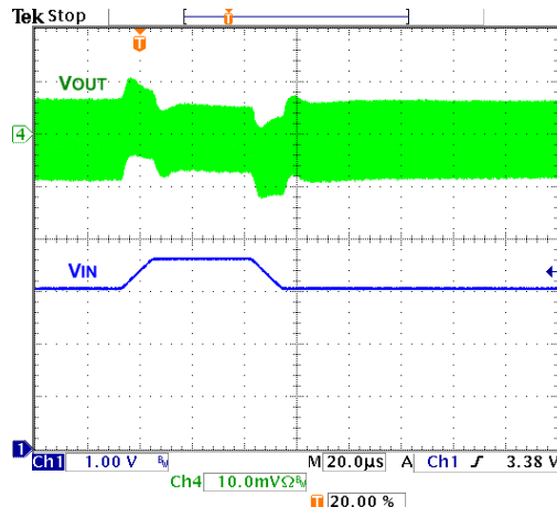
Figure 19 Line Transient, 200mA Load, 10µs Step
