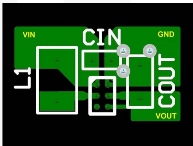
Figure 32 WLCSP Suggested Layout (Top View)
