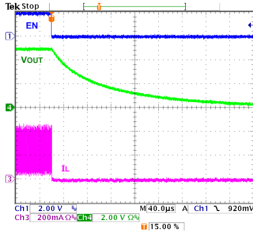
Figure 23 Shutdown, 33Ω Load
