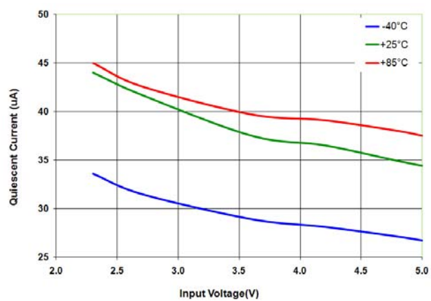
Figure 11 Quiescent Current
