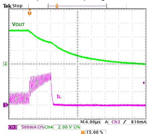
Figure 24 Overload Protection
