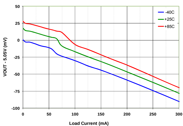
Figure 9 Load Regulation vs. Temperature, 3.6V IN
