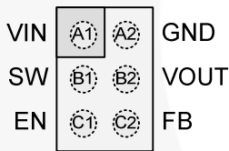
Figure 3. WLCSP (Top View)
