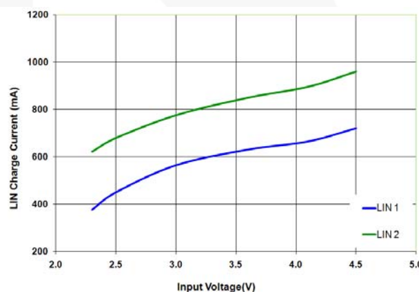
Figure 29. LIN Mode Current vs. V_{IN}
