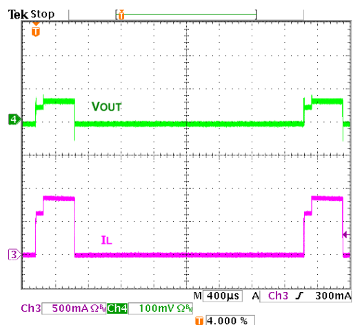
Figure 25 Short-Circuit Response
