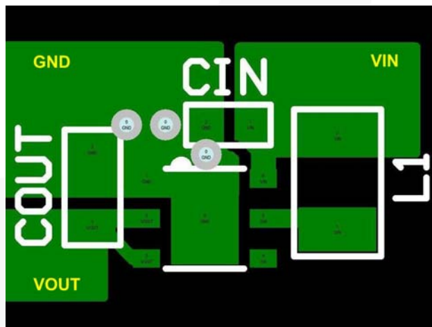
Figure 33 UMLP Suggested Layout (Top View)
