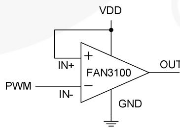
Figure 46. Dual-Input Driver Enabled, Inverting Configuration
