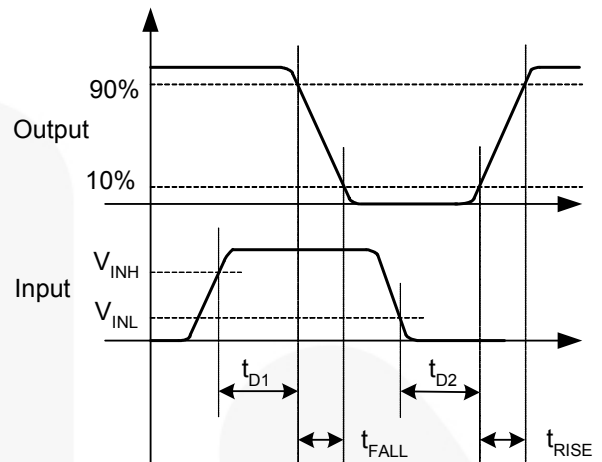
Figure 8. Inverting
