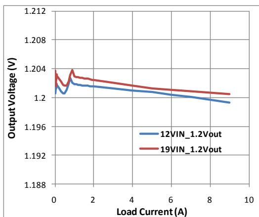
Figure 12. Load Regulation
