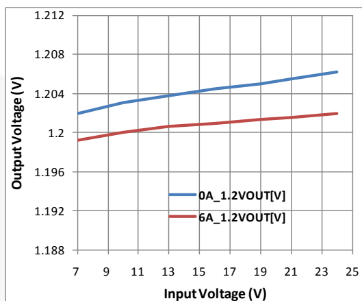
Figure 13. Line Regulation
