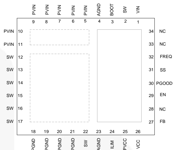
Figure 5. Pin Assignments(Top View)
