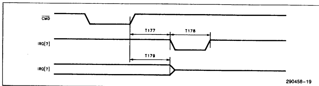
Figure 11-16. Interrupt Timing
