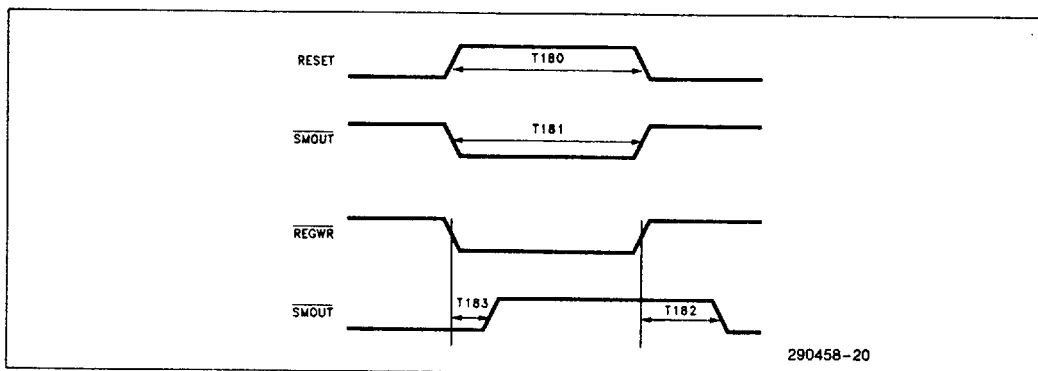
Figure 11-17. SMOUT Timing
