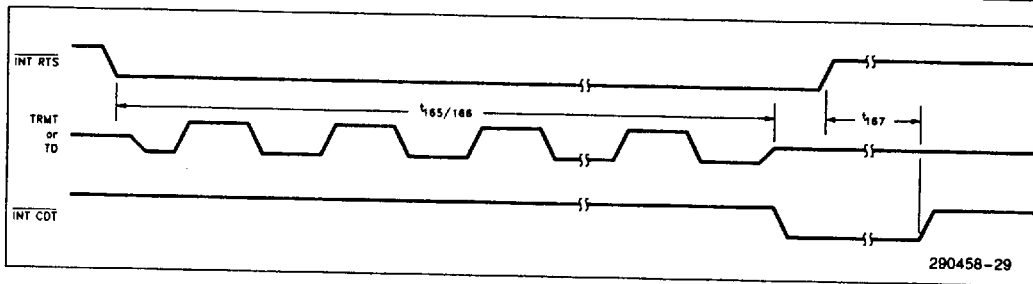
Figure 11-26. Jabber Timings
