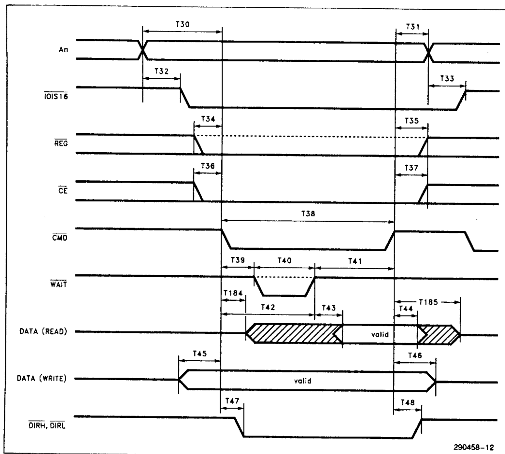
Figure 11-8. PCMCIA Cycle
