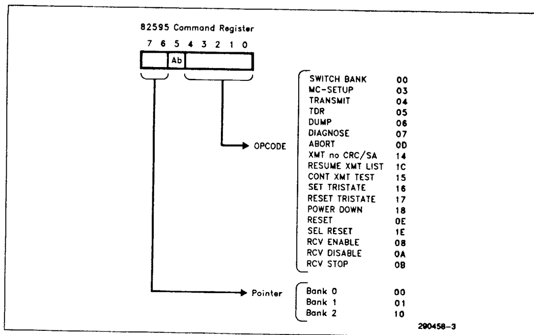
Figure 5-2. 82595 Command Interface
