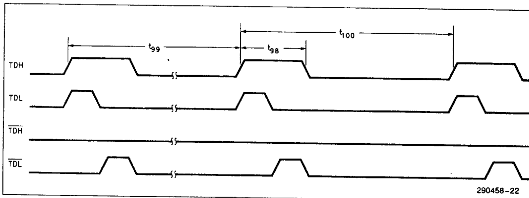
Figure 11-19. TPE Transmit Timings (Link Test Pulse)
