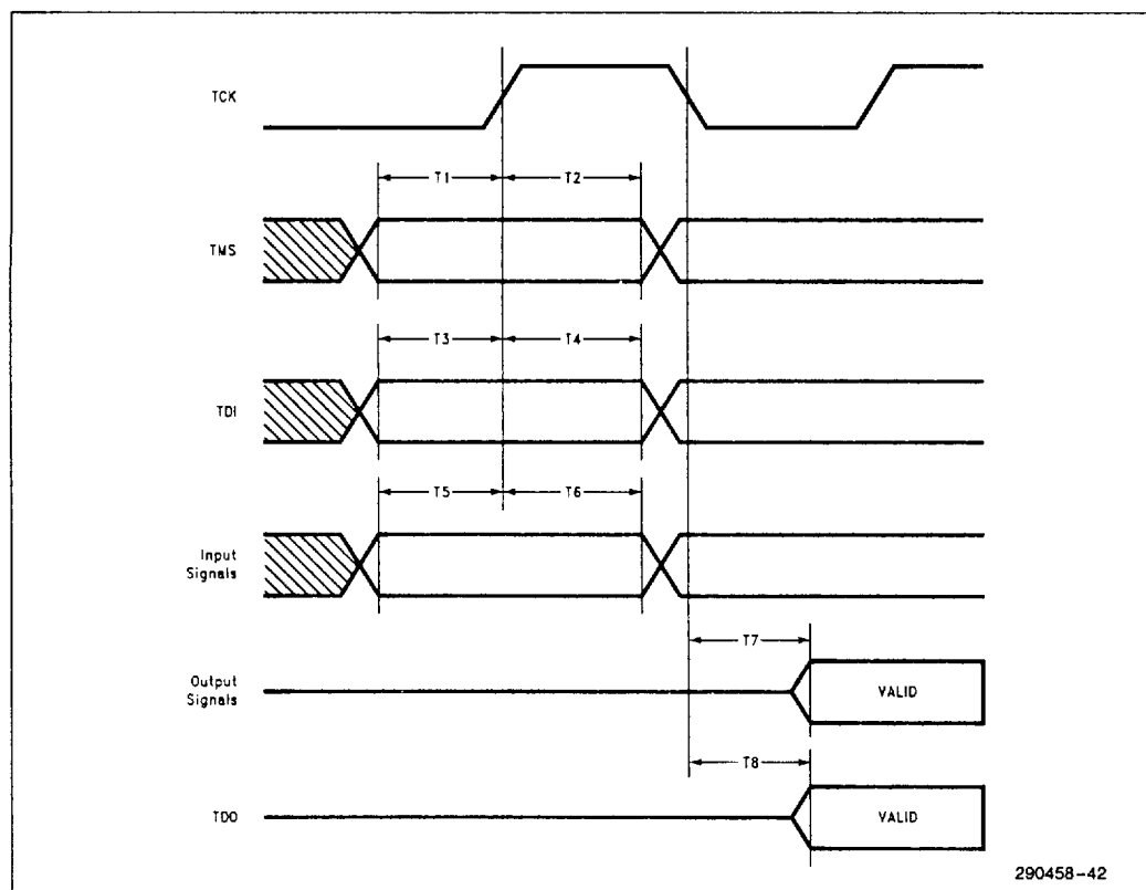
Figure 11-18. 82595 JTAG Timing
