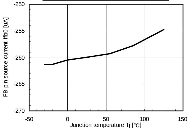
FB pin source current vs Junction temperature(Tj)
