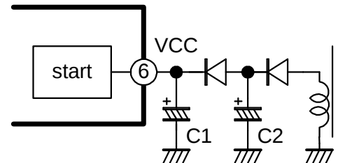
Fig.16 VCC circuit
