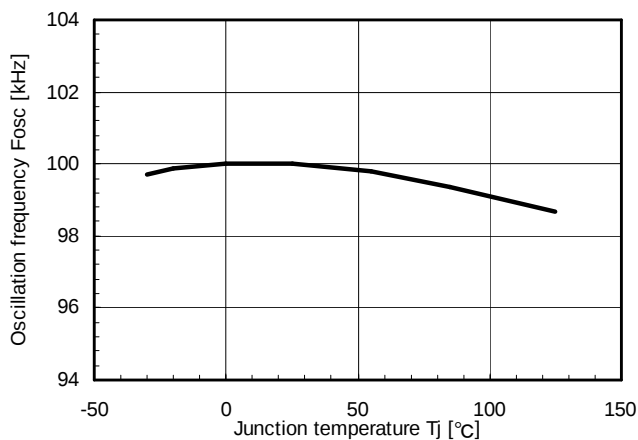
Oscillation frequency vs Junction temperature (Tj)
