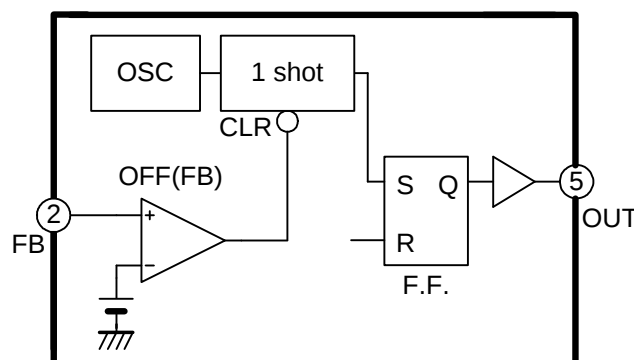
Fig.9 Output shutdown function of FB pin
