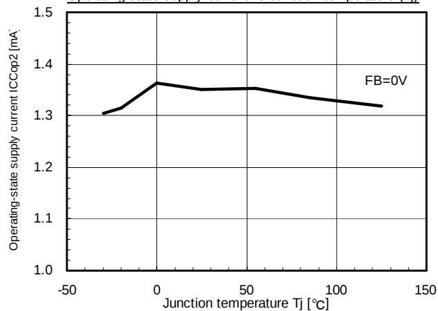
Operating-state supply current vs Junction temperature (Tj)
