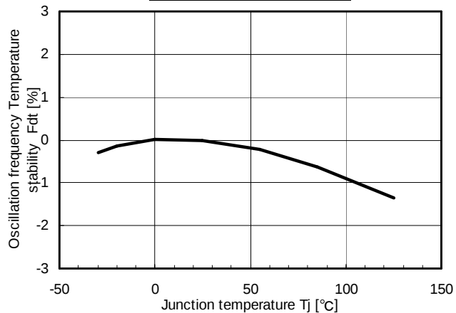
Fdt vs Junction temperature (Tj)
