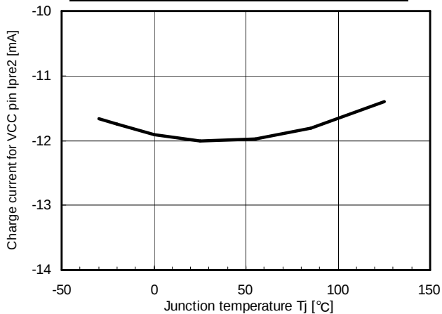
Charge current for VCC pin vs Junction temperature (Tj)
