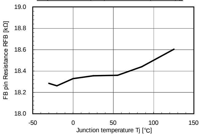
FB pin Resistance (RFB) vs Junction temperature (Tj)
