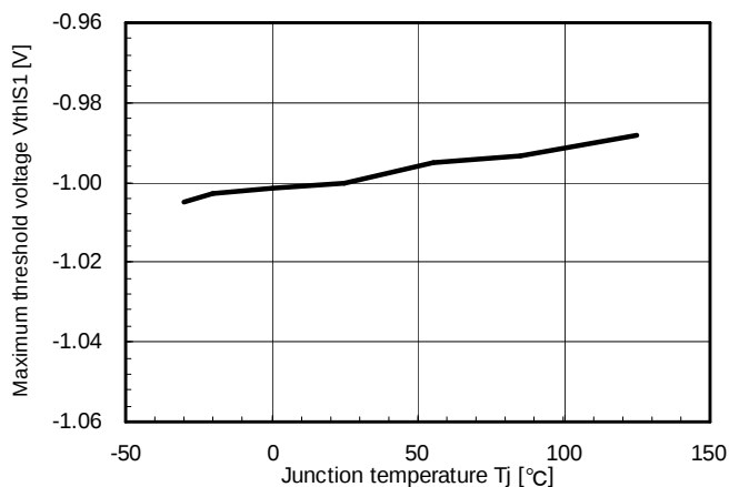
Maximum threshold voltage vs Junction temperature (Tj)
