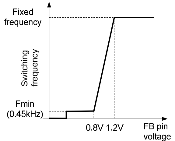
Fig.4 Oscillation frequency
