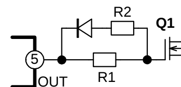
Fig.18 Gate drive circuit (2)
