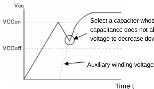
Fig.14 VCC terminal voltage at startup
