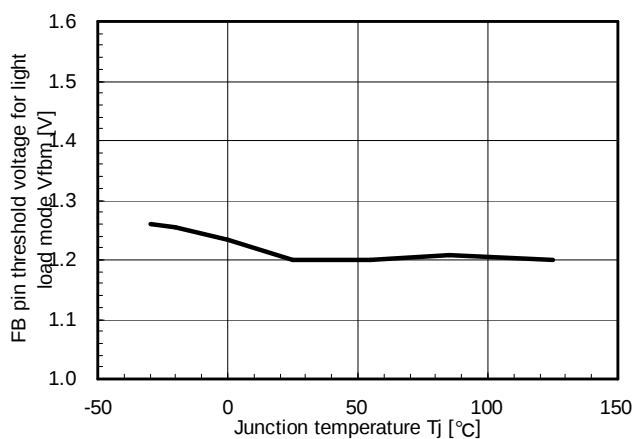
Vfbm vs Junction temperature(Tj)
