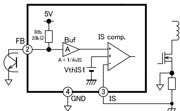
Fig.7 Current comparator
