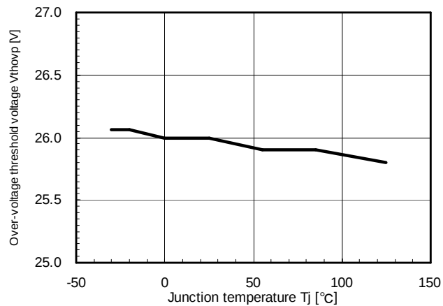
Vthovp vs Junction temperature (Tj)
