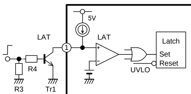
Fig.19. Latch shutdown function by an external signal
