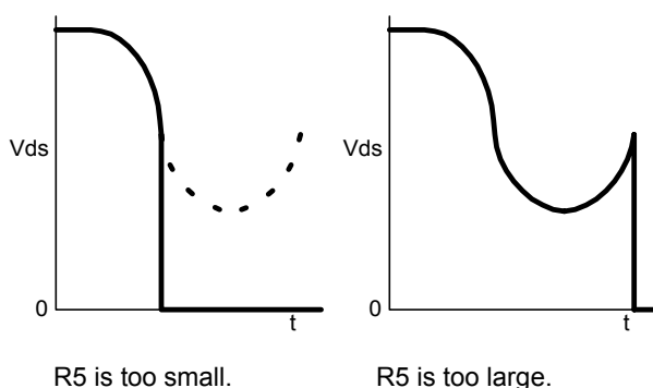
Fig.18 Vds waveform at turn on (with inadequate R5)
