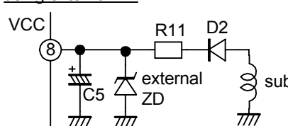
Fig.15 Vcc clamp circuit
