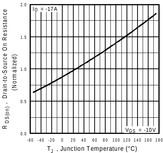
Fig 4. Normalized On-Resistance
