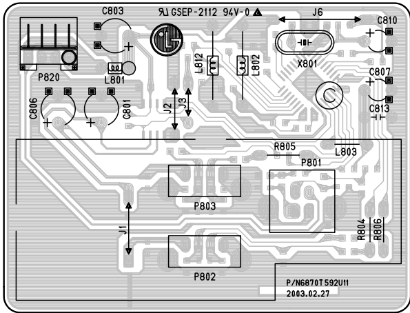
5. USB BOARD (Component Side)
