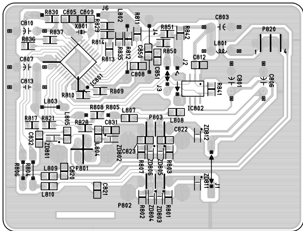
6. USB BOARD (Solder Side)
