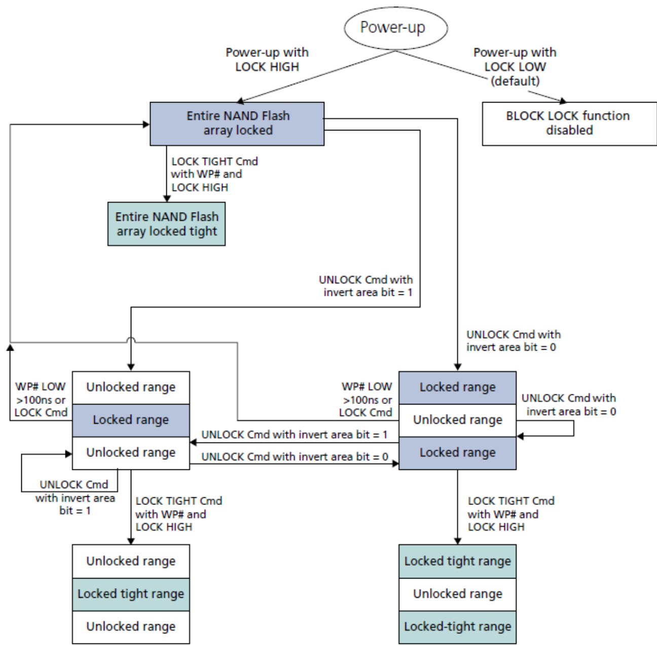
BLOCK LOCK Flowchart
