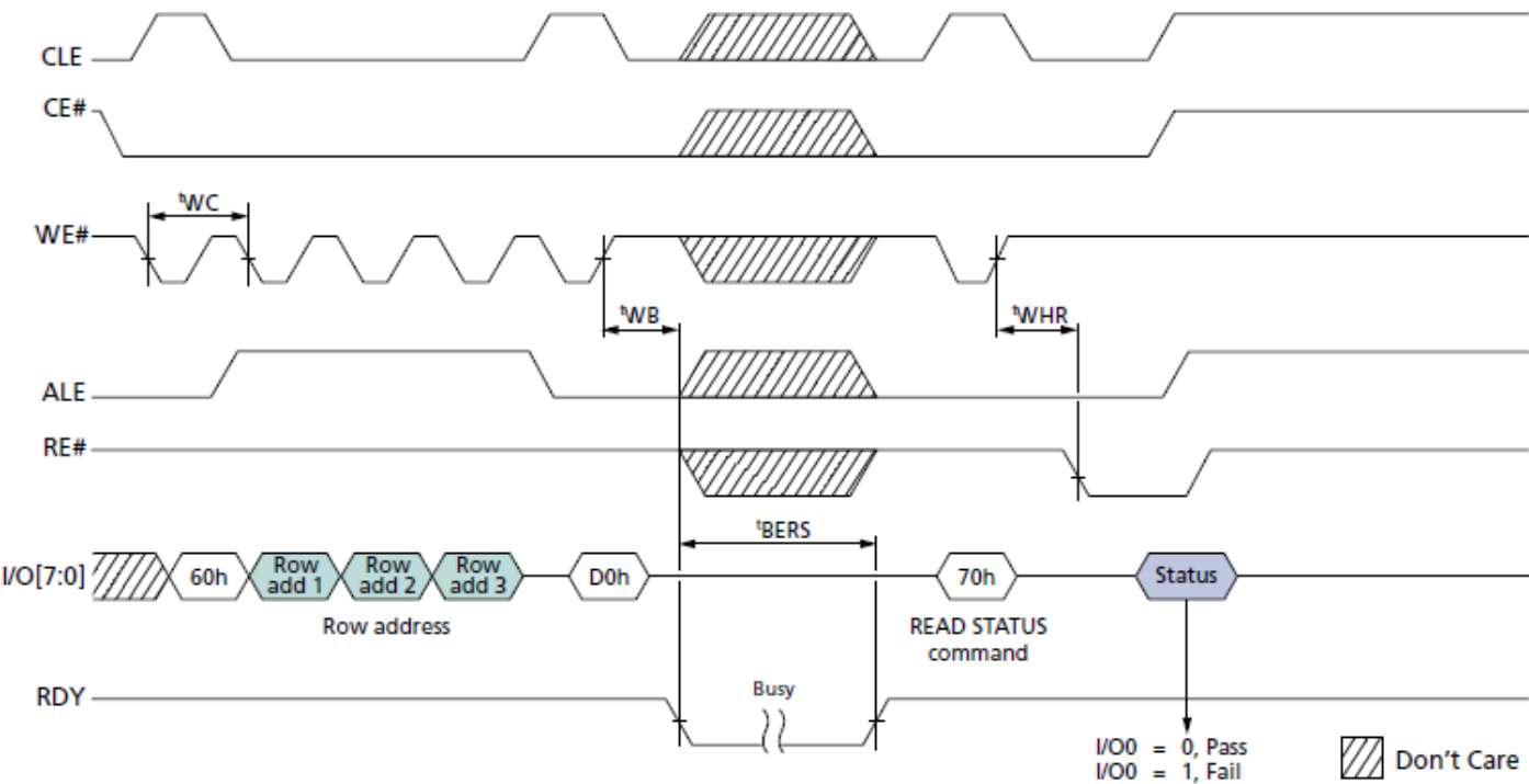
ERASE BLOCK Operation
