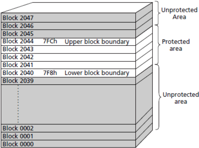
Flash Array Protected: Invert Area Bit = 1
