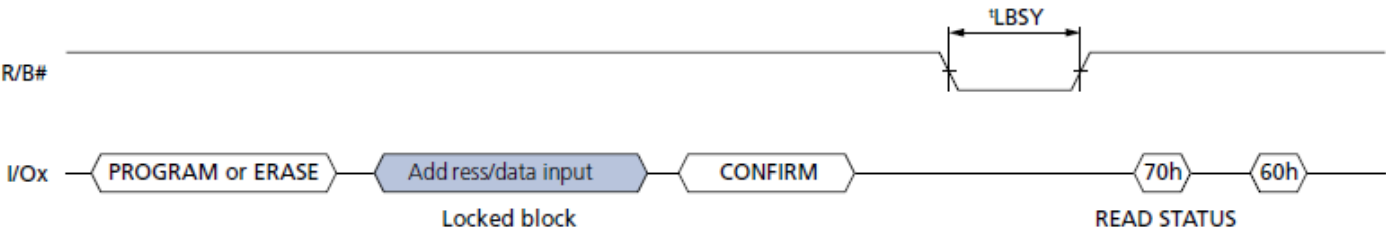
PROGRAM/ERASE Issued to Locked Block
