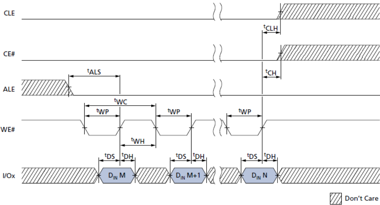
Asynchronous Data Input Cycles
