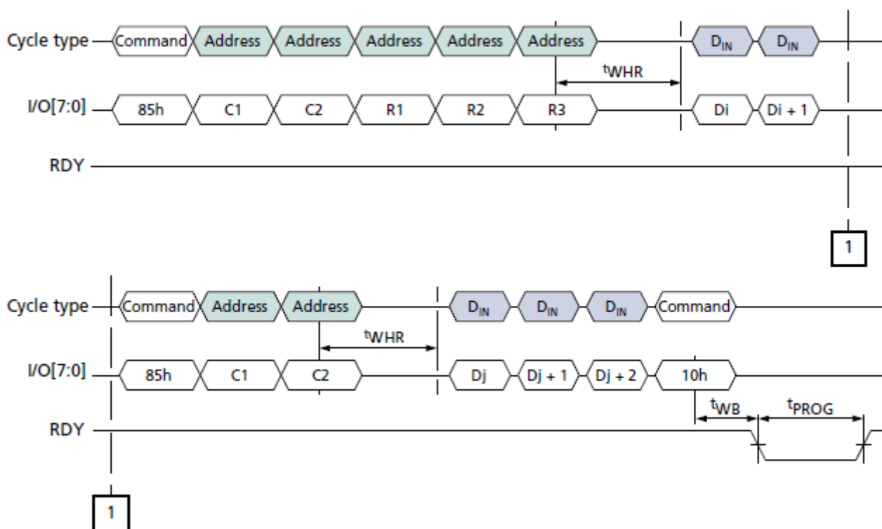
PROGRAM FOR INTERNAL DATA MOVE (85h-10h) with RANDOM DATA INPUT (85h)
