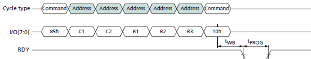
PROGRAM FOR INTERNAL DATA MOVE (85h–10h) Operation
