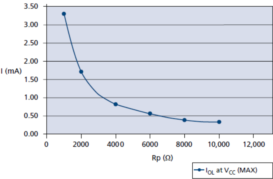
I_{OL} vs. R_p
