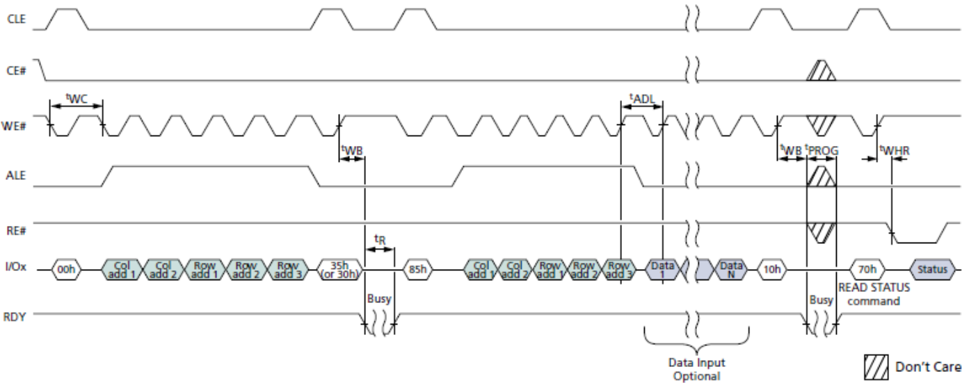
INTERNAL DATA MOVE
