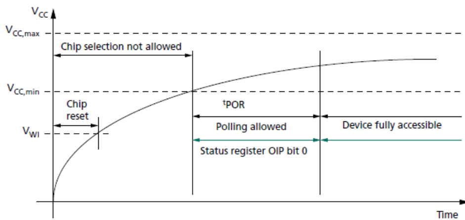
SPI Power-Up
