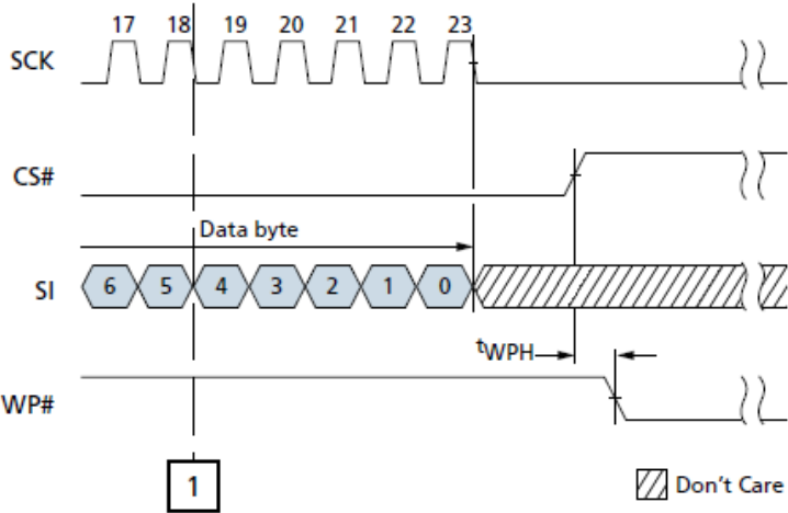
WP# Timing
