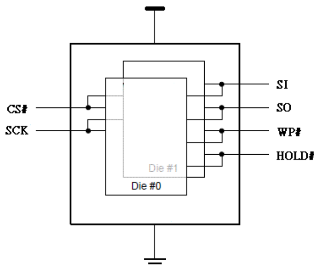
A Brief Sketch of 2Gb Device
