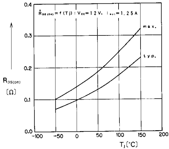
On-Stage Resistance
