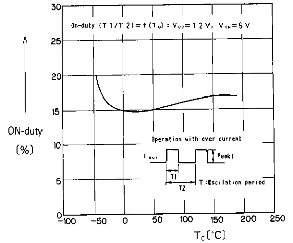
Over-Current protection
