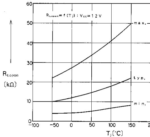
Open-Load Detection
