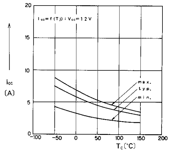
Over-Current Detection
