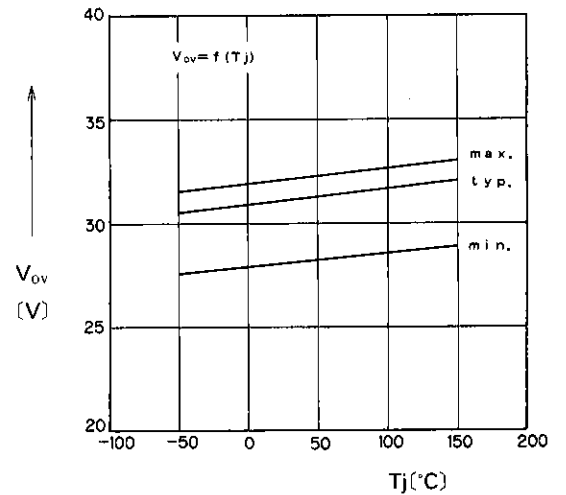
Over-Voltage Detection
