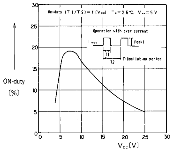
Over-Current protection
