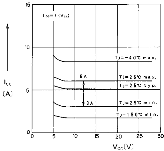
Over-Current Detection
