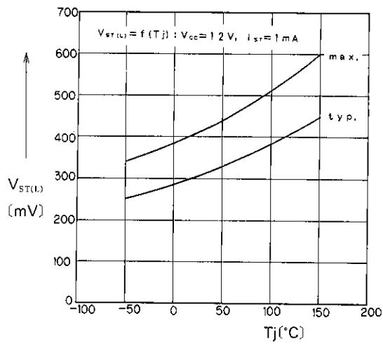
Status Voltage
