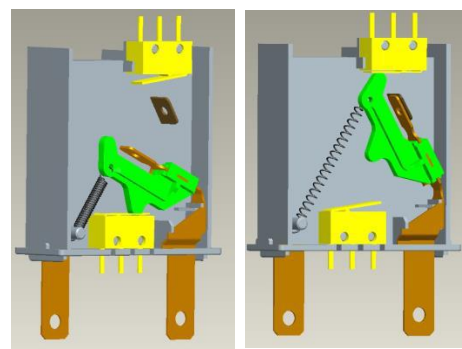
F34V internal structure
