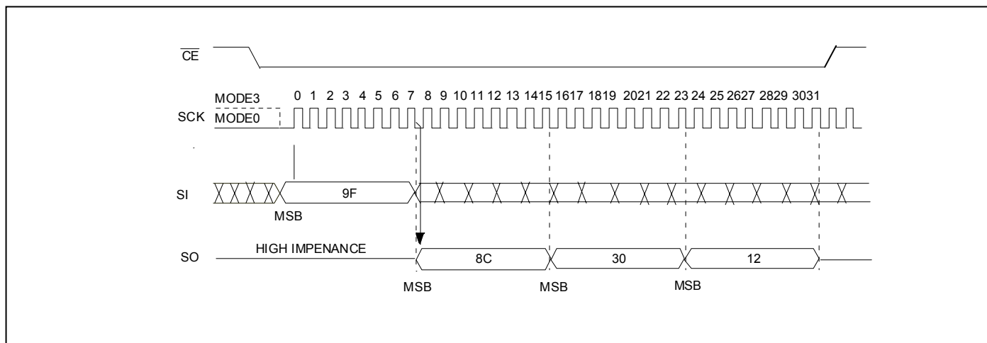
Figure 18: JEDEC Read-ID Sequence
