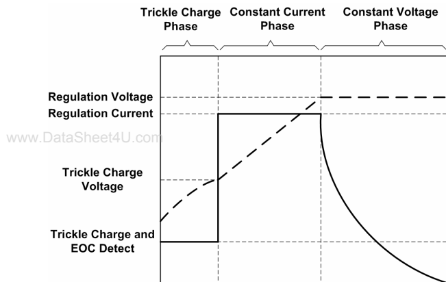
Figure 5. Typical Charge Profile
