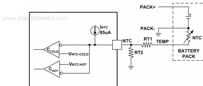
Figure 8. Temperature Sensing Thresholds
