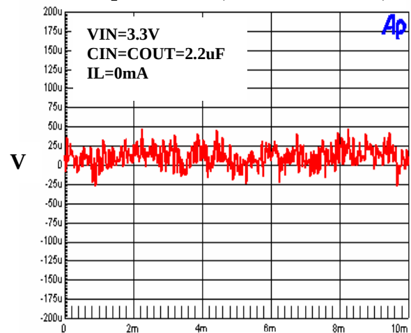
Output1 Noise (10Hz to 100KHz)
