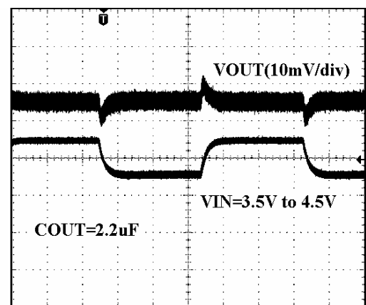
Line Transient Response (COUT=2.2uF)
