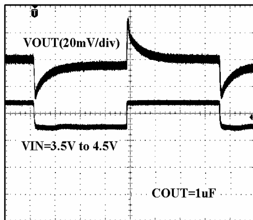
Line Transient Response (COUT=1uF)
