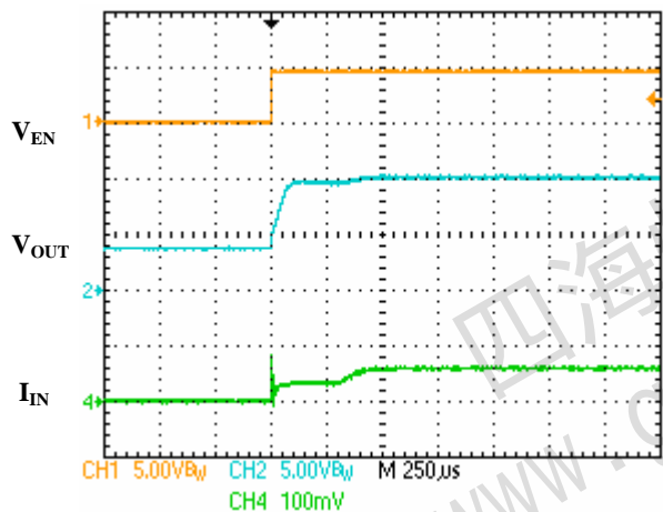
Startup Waveforms
