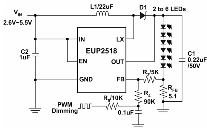
Figure 5. Filtered PWM Signal for LED Dimming Control
