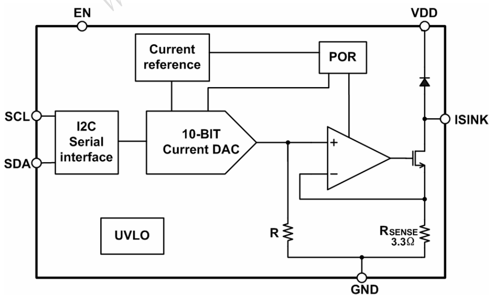
Figure 2. Block Diagram
