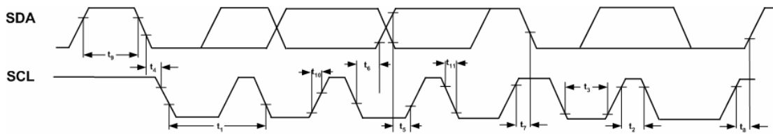
Figure 14. I²C Interface timing Diagram
