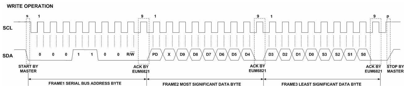
Figure 16. Write Operation
