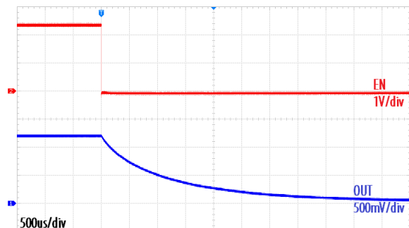
Shutdown Waveform at No Load, V_{OUT} = 1.2\text{V}
