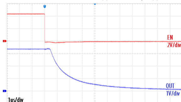
Shutdown Waveform with R_{OUT} = 3.3\Omega , V_{OUT} = 3.3\text{V}
