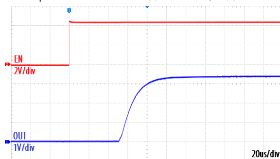
Start-Up Waveform with R_{OUT} = 3.3\Omega , V_{OUT} = 3.3\text{V}
