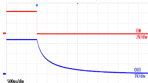
Shutdown Waveform at No Load, V_{OUT} = 3.3\text{V}
