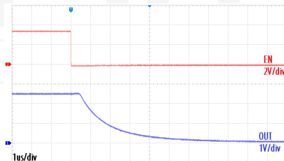
Shutdown Waveform with R_{OUT} = 2.5\Omega , V_{OUT} = 2.5\text{V}
