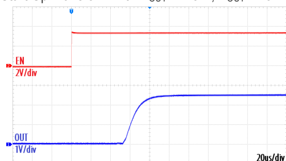
Start-Up Waveform with R_{OUT} = 2.5\Omega , V_{OUT} = 2.5\text{V}
