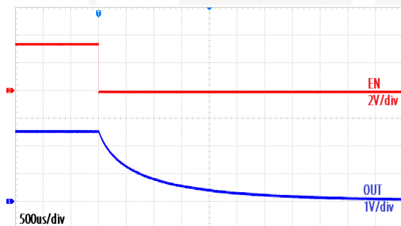
Shutdown Waveform at No Load, V_{OUT} = 2.5\text{V}
