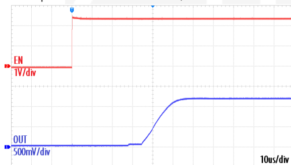
Start-Up Waveform at No Load, V_{OUT} = 1.2\text{V}
