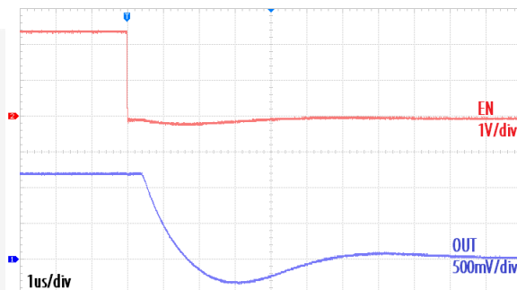
Shutdown Waveform with R_{OUT} = 1.2\Omega , V_{OUT} = 1.2\text{V}
