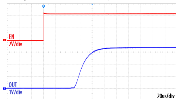
Start-Up Waveform at No Load, V_{OUT} = 3.3\text{V}
