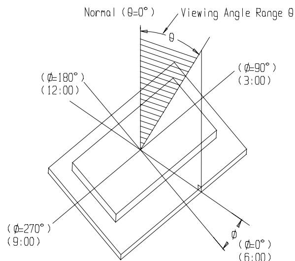
Figure 6. Definition of contrast ratio 'Cr'. & viewing angle range ' \theta '.
