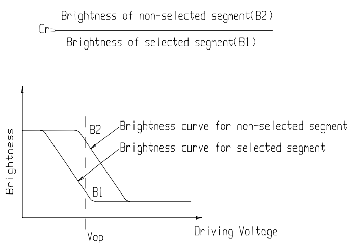
Figure 6. Definition of contrast ratio 'Cr'. & viewing angle range ' \theta '.
