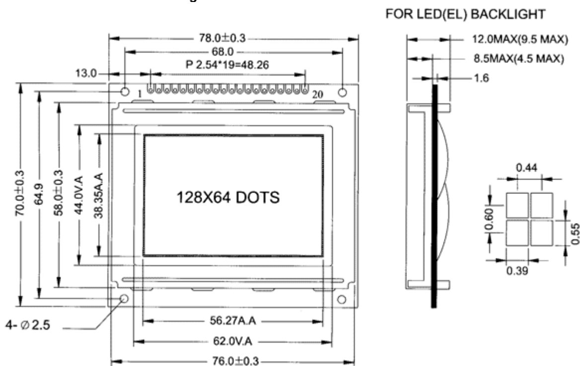
Figure 1. External Dimensions
