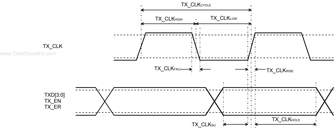
Figure 22. MII 10Base-T Transmit Timing
