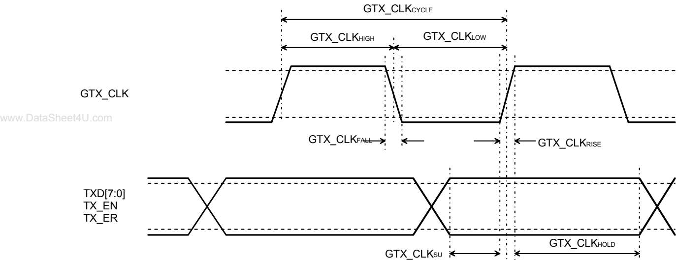
Figure 14. GMII 1000Base-T Transmit Timing
