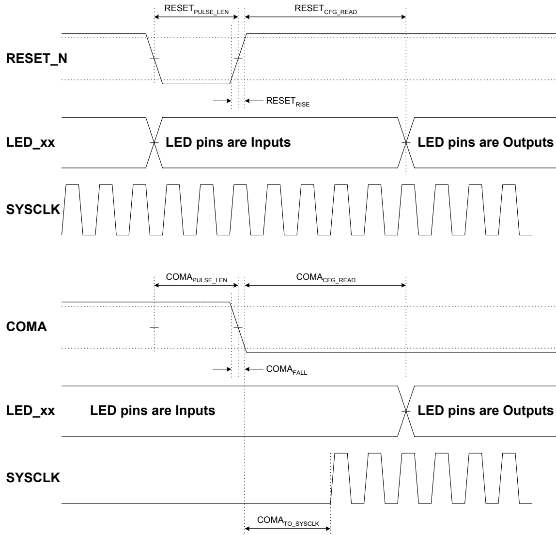
Figure 25. Reset Timing
