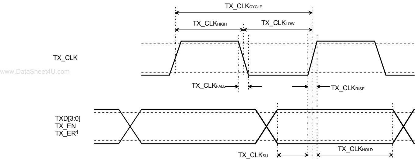
Figure 20. MII 100Base-TX Transmit Timing
