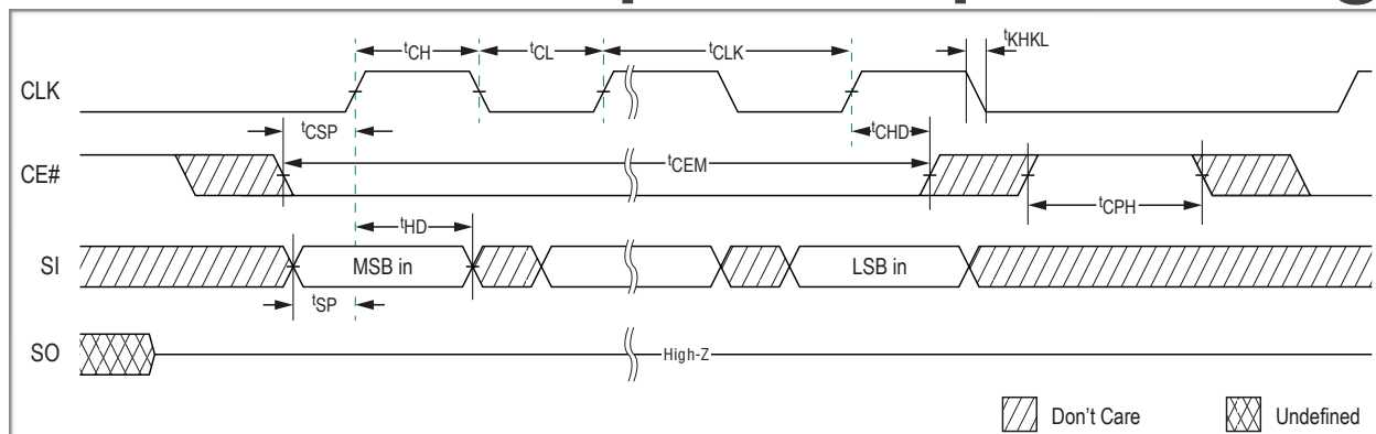
Figure 12-1. Input Timing
