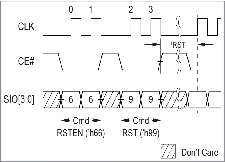
Figure 9-2. QPI Reset
