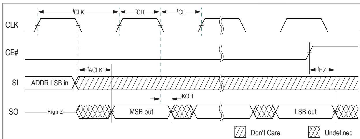
Figure 12-2. Output Timing
