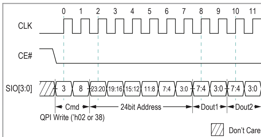
Figure 8-3. QPI Write
