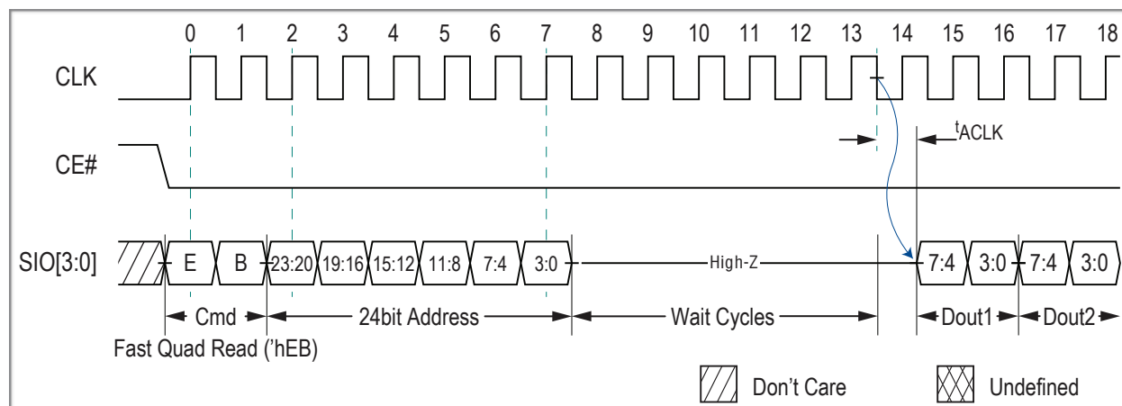
Figure 8-2. QPI Fast Quad Read 'hEB (max freq 133 MHz)
