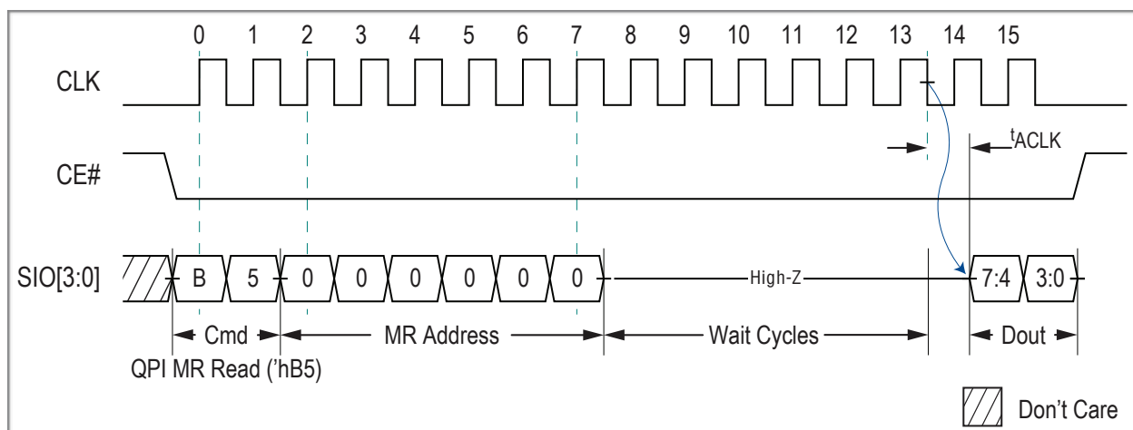
Figure 6-3. QPI MR Read 'hB5'
