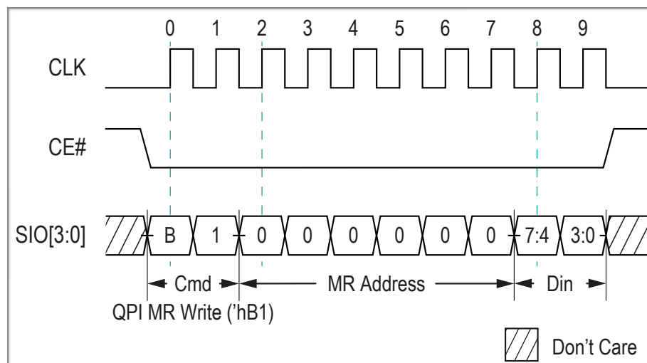
Figure 6-4. QPI MR Write 'hB1'
