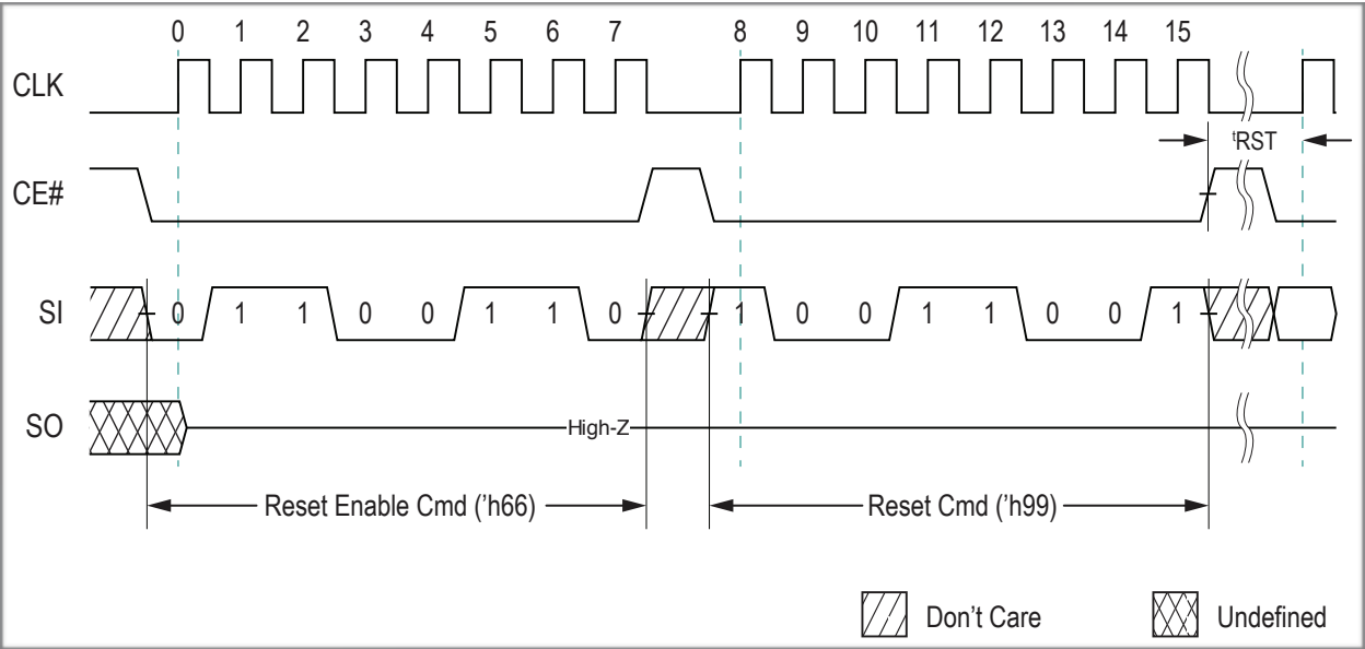
Figure 9-1. SPI Reset
