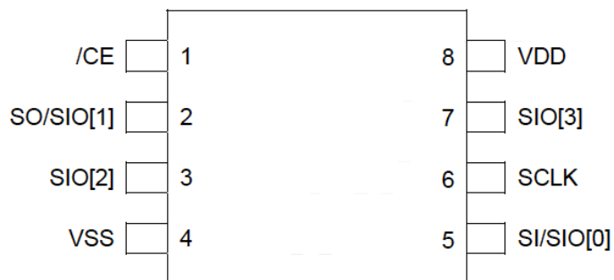
Figure 2-1. Pin Layout
