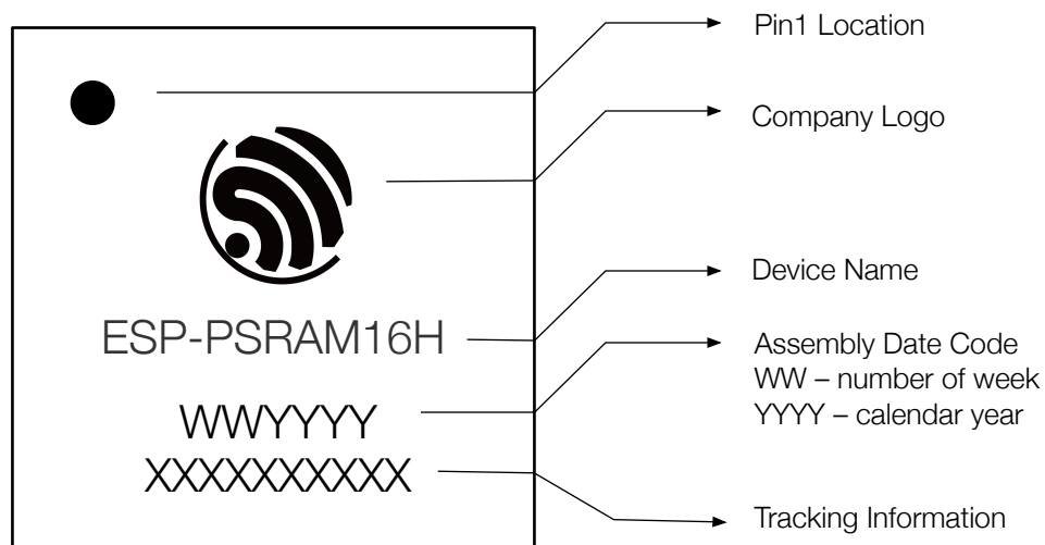
Figure A-1. Device Marking of ESP-PSRAM16H
