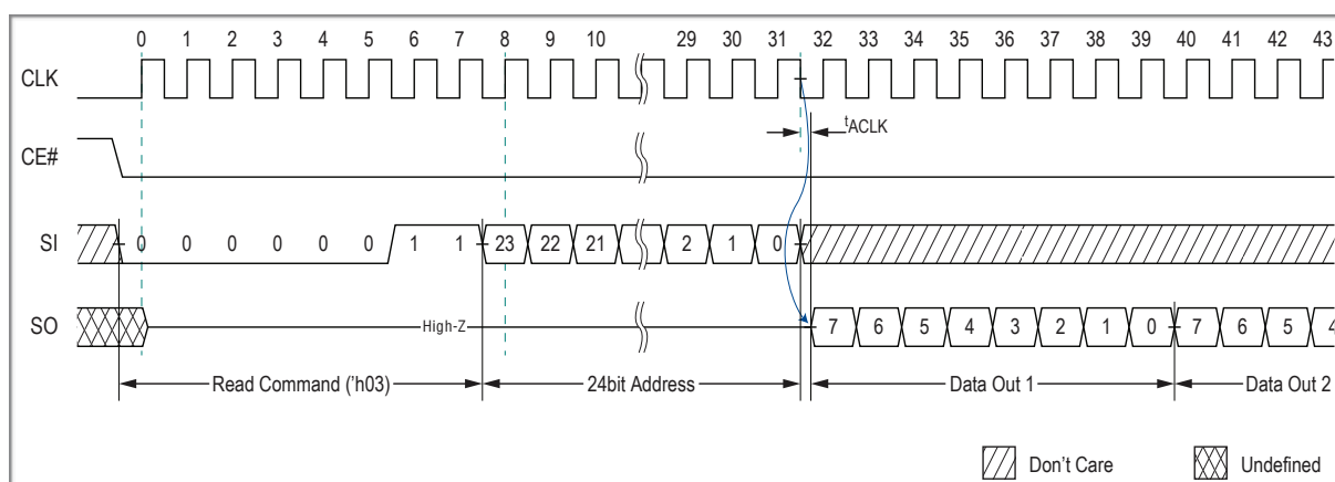
Figure 7-1. SPI Read 'h03 (max freq 33 MHz)
