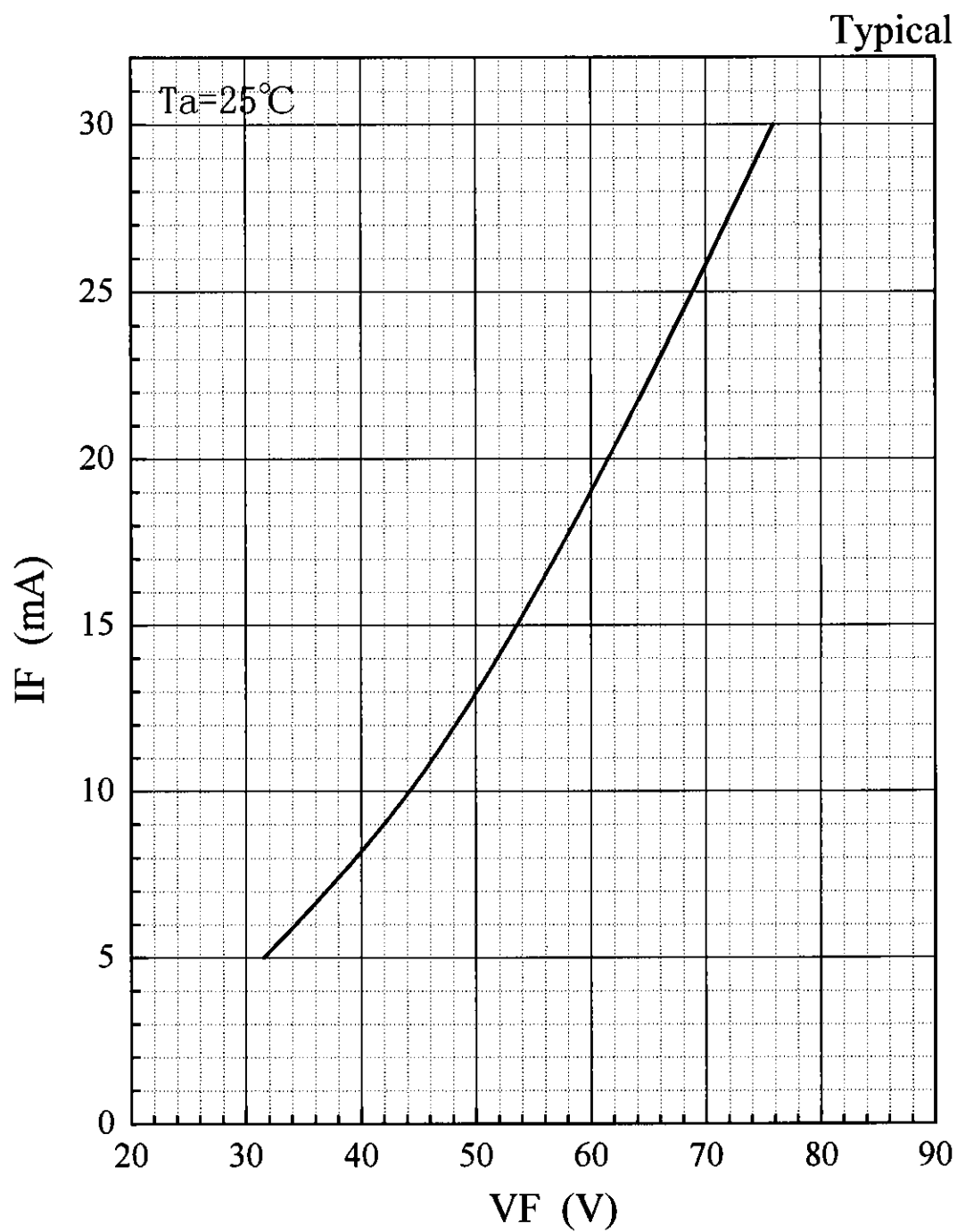
Fig.1 Forward characteristic[VF-IF]
