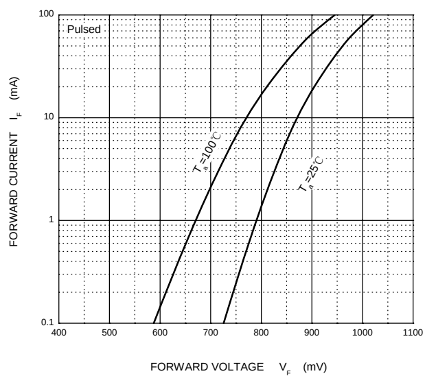
Forward Characteristics
