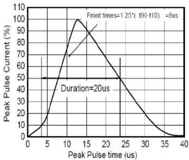
8/20us waveform
