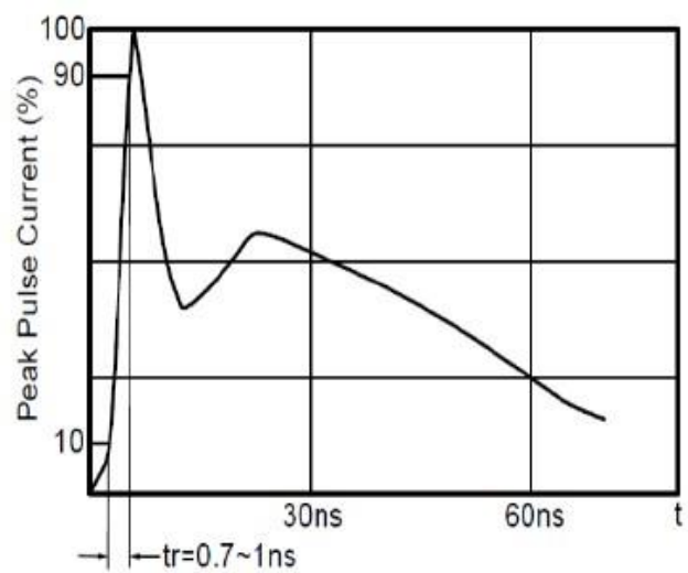
IEC61000-4-2 waveform
