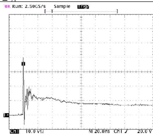
FIG.1-POSITIVE 8KV CONTACT PER IEC6100-4-2
