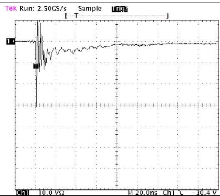
FIG.2-NEGATIVE 8KV CONTACT PER IEC6100-4-2-SESD5L5V 61000-4-2
