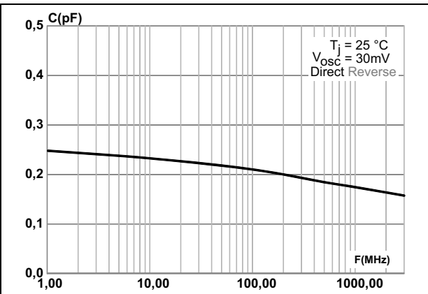
Figure 4. Junction capacitance versus frequency (typical values)
