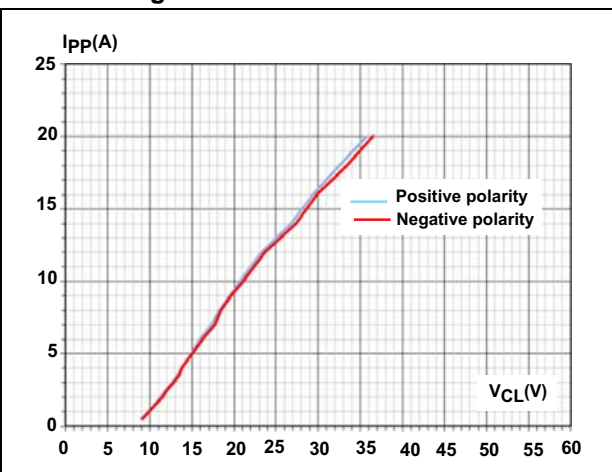
Figure 8. TLP measurements
