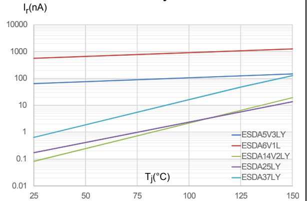
Figure 6: Relative variation of leakage current at V_R = V_{RM} versus junction values
