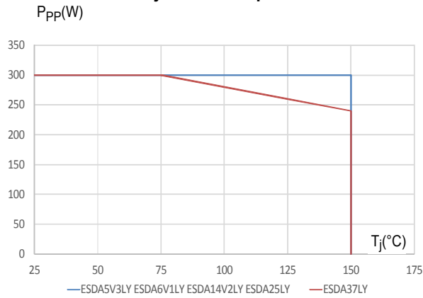
Figure 3: Variation of peak pulse power versus initial junction temperature
