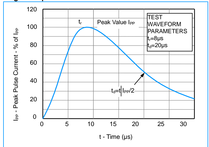
Fig5. 8x20 \mu s Pulse Waveform
