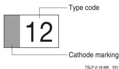
Figure 12 PG-TSLP-2-18: Marking (example)
