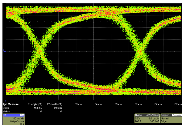
Without ESD8104
