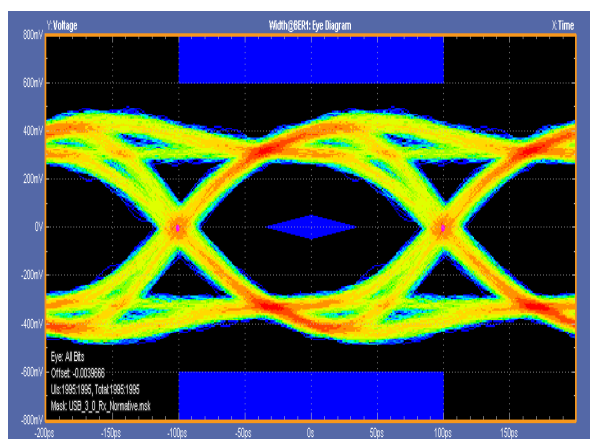
Without ESD8104
