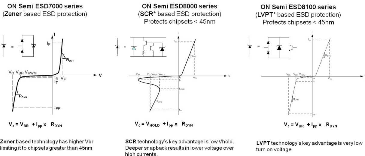
Figure 17. onsemi's Low-cap ESD Technology Portfolio
