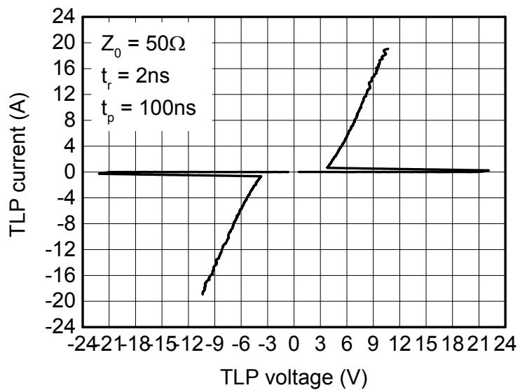
TLP Measurement
